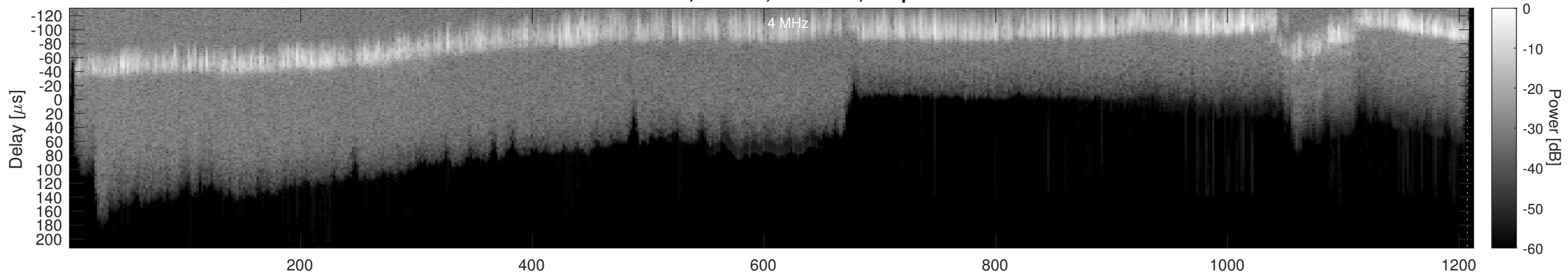
Orbit 15732, Window, Channel 2, Optimized
