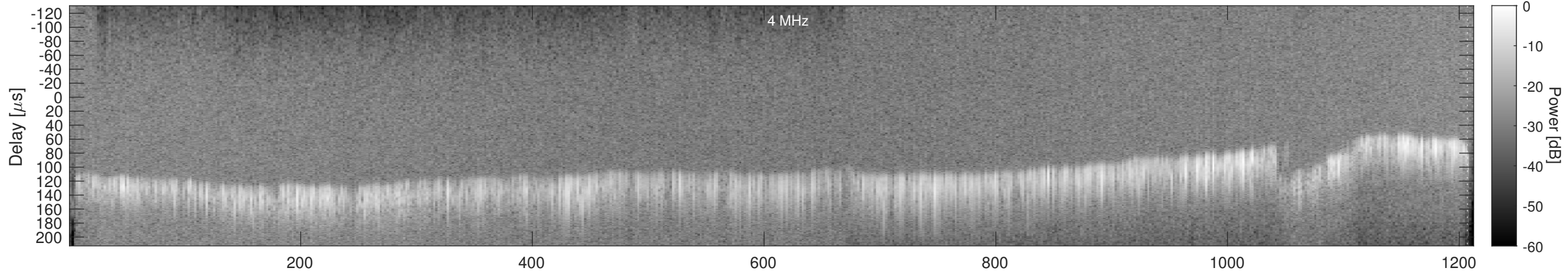
Orbit 15732, Window, Channel 2, Chapman
