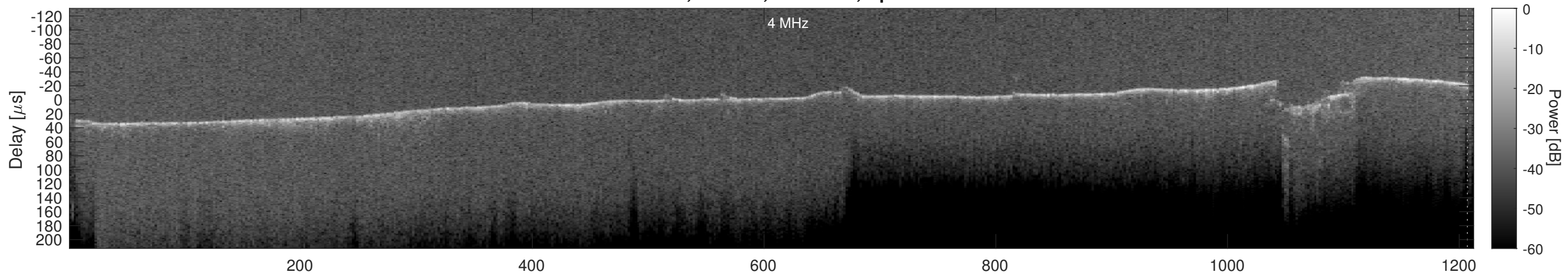
Orbit 15732, Cluttergram
