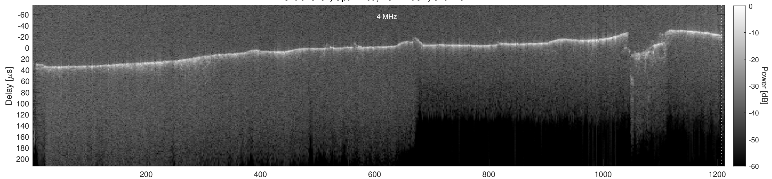
Orbit 15732, Cluttergram
