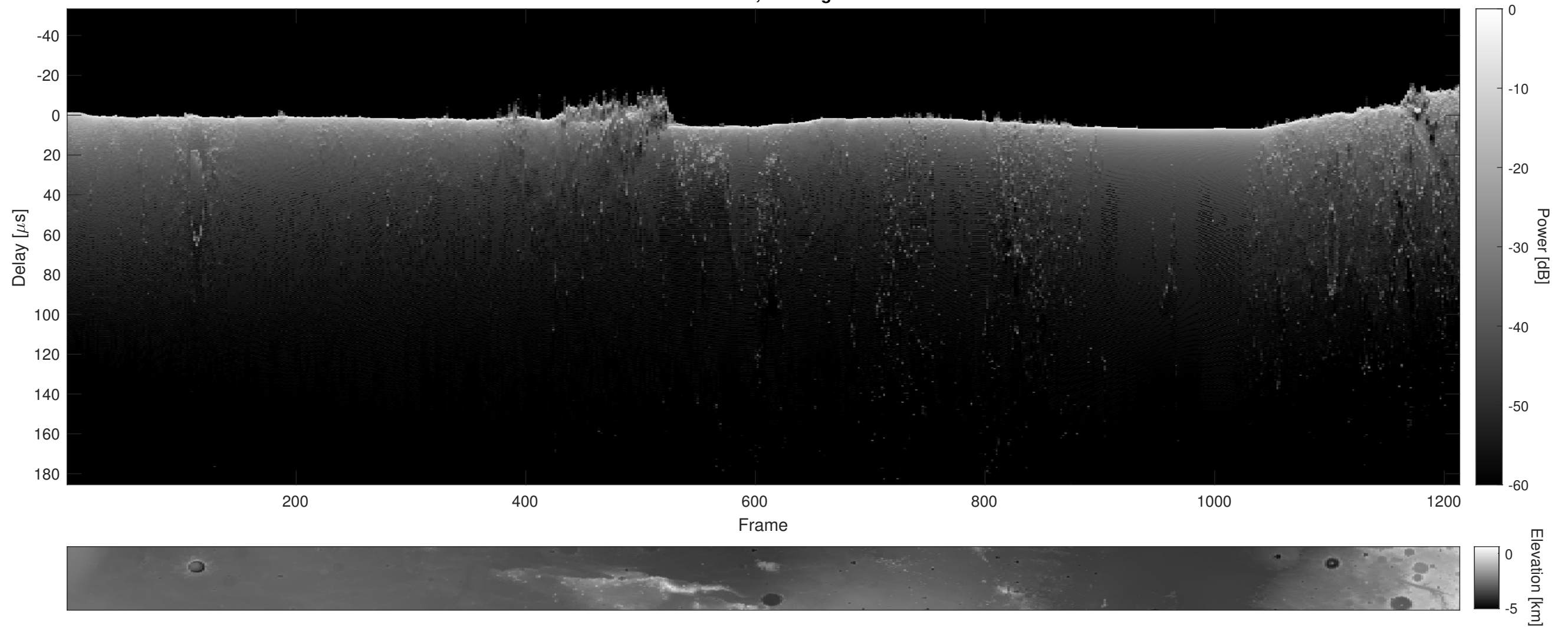
Orbit 15733, Cluttergram
