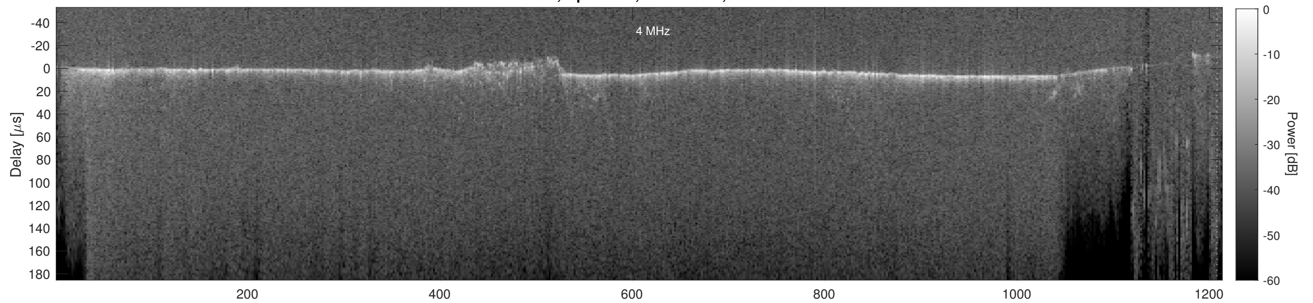
Orbit 15733, Cluttergram
