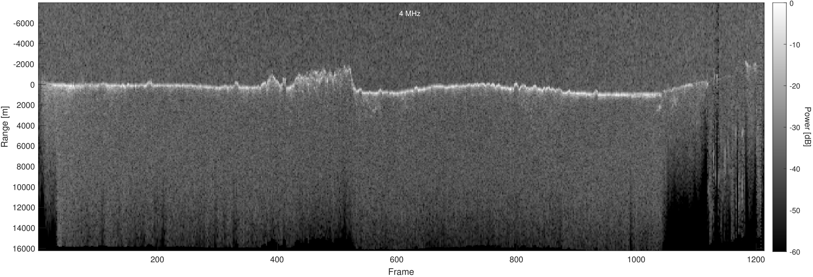
Orbit 15733, Optimized, Window, Depth-Corrected, Channel 2
