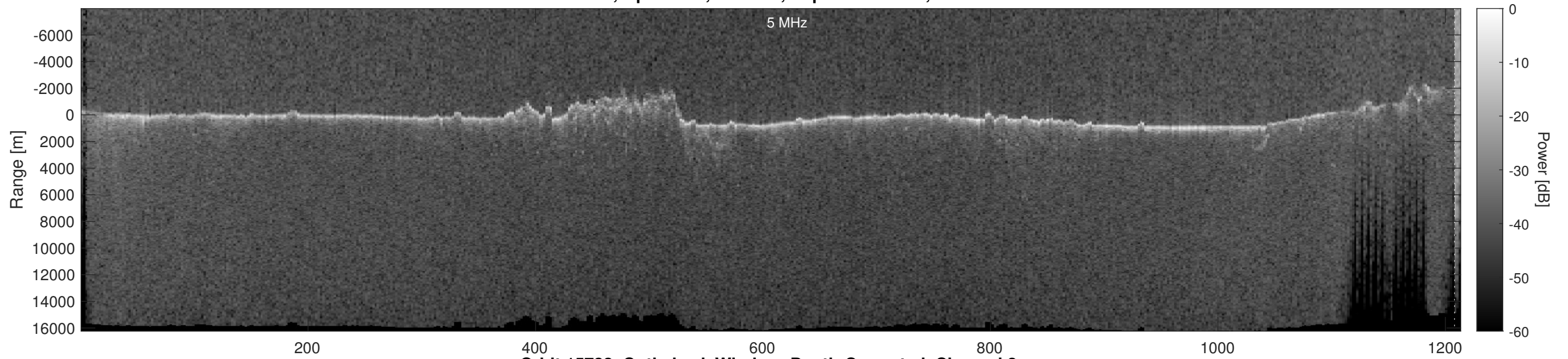
Orbit 15733, Optimized, Window, Depth-Corrected, Channel 2
