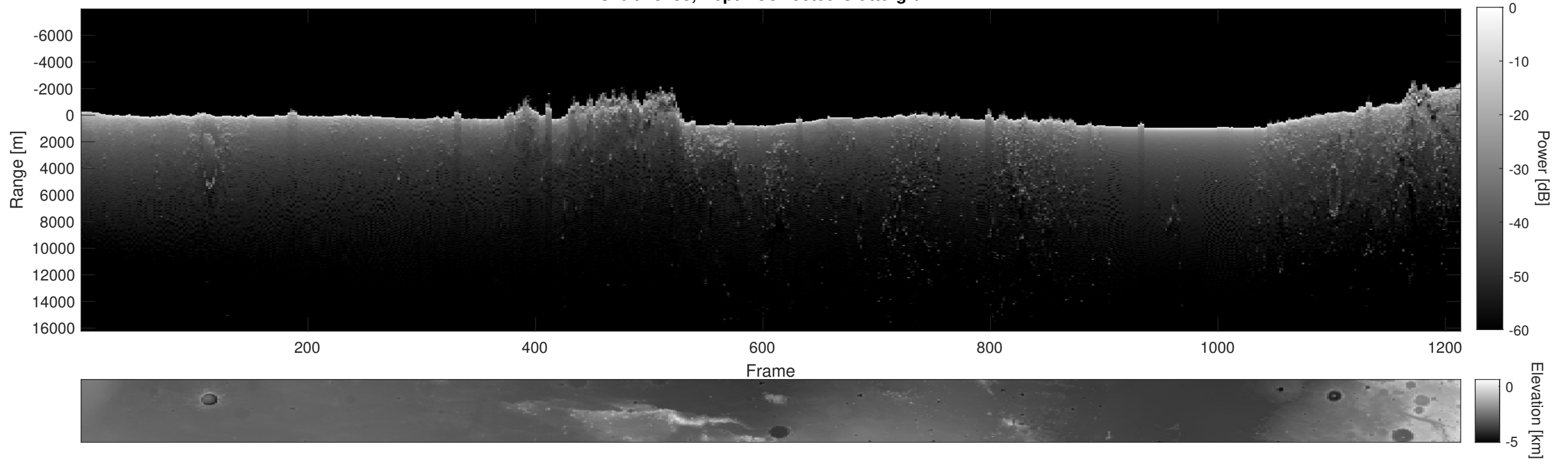
Orbit 15733, Depth-Corrected Cluttergram
