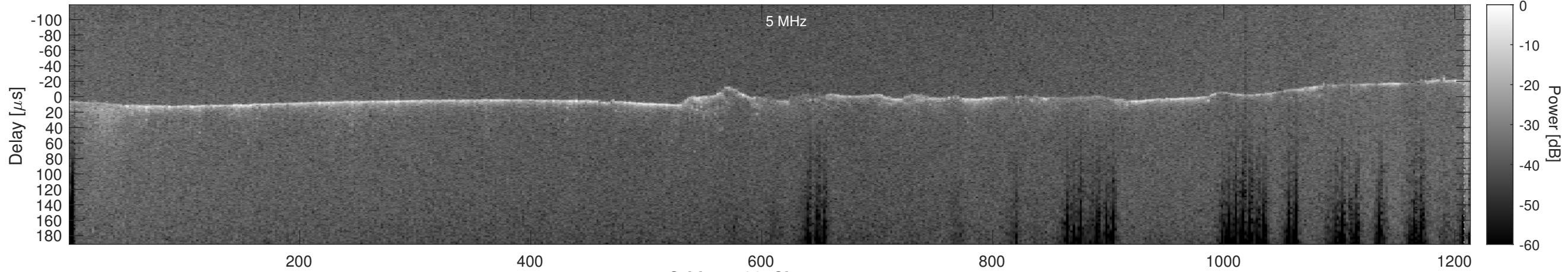
Orbit 15736, Cluttergram
