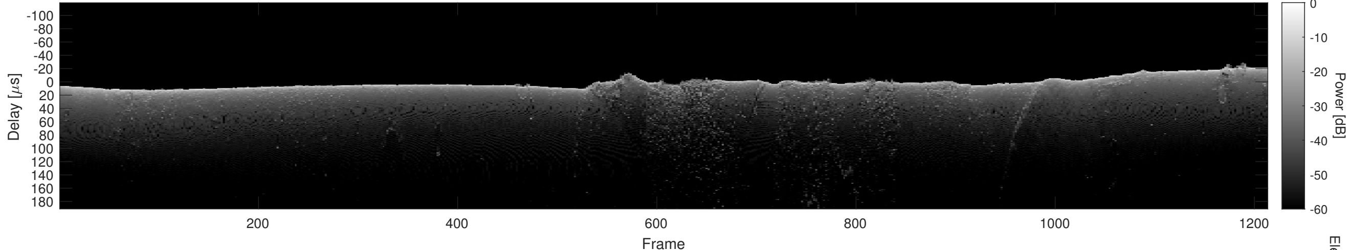
Orbit 15736, Cluttergram
