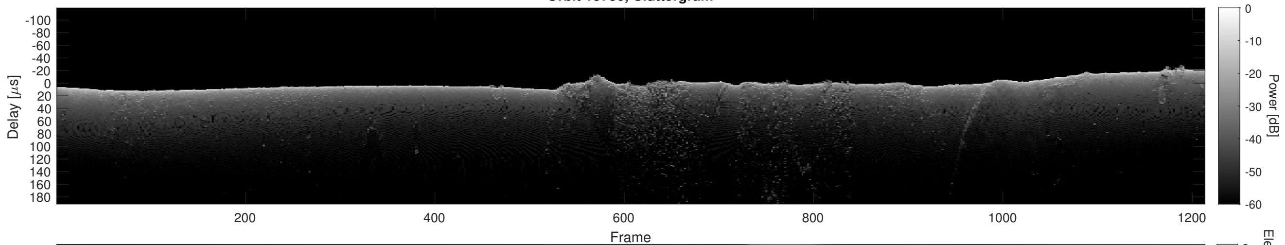
Orbit 15736, Cluttergram
