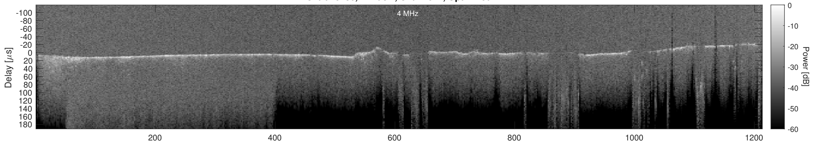
Orbit 15736, Cluttergram
