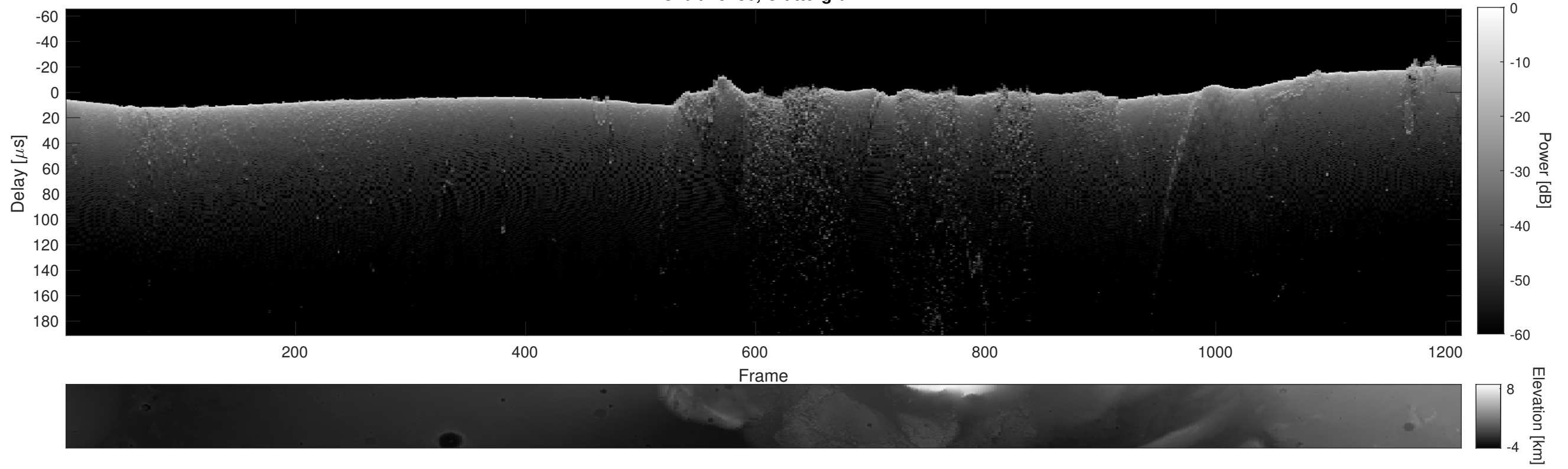
Orbit 15736, Cluttergram
