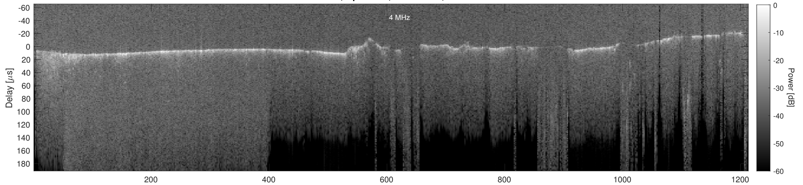
Orbit 15736, Cluttergram
