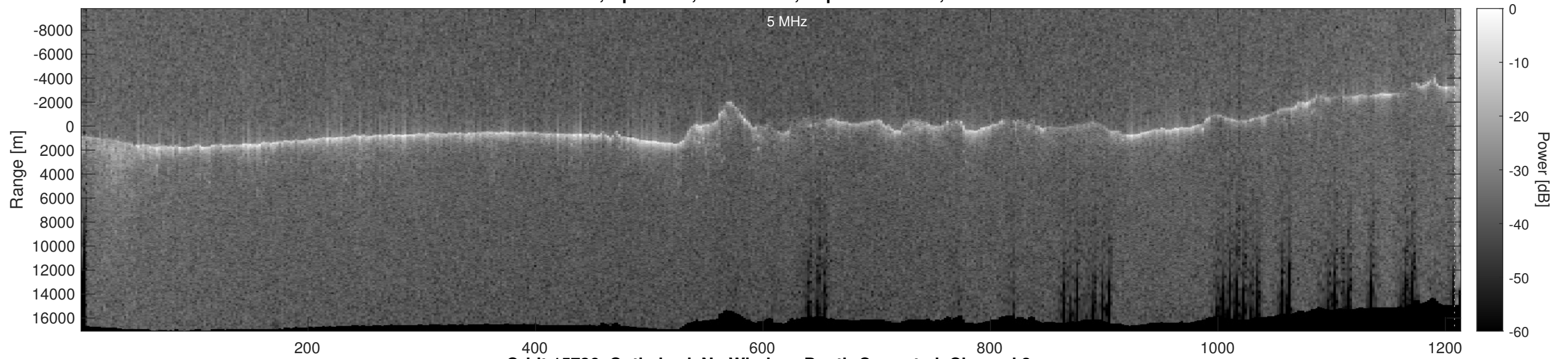
Orbit 15736, Optimized, No Window, Depth-Corrected, Channel 2
