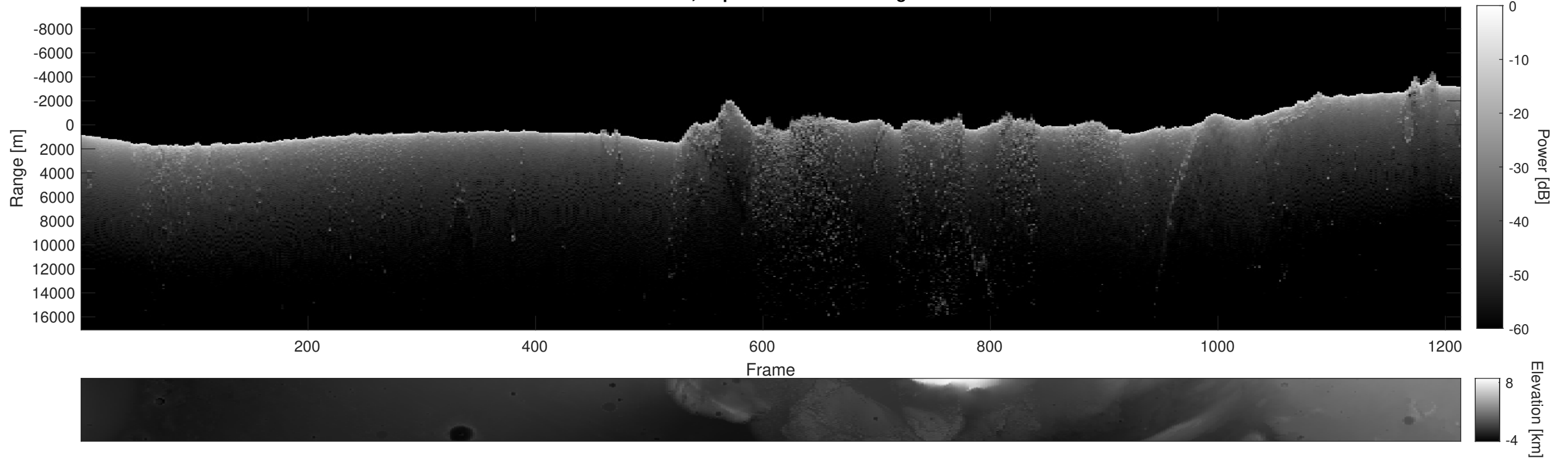
Orbit 15736, Depth-Corrected Cluttergram
