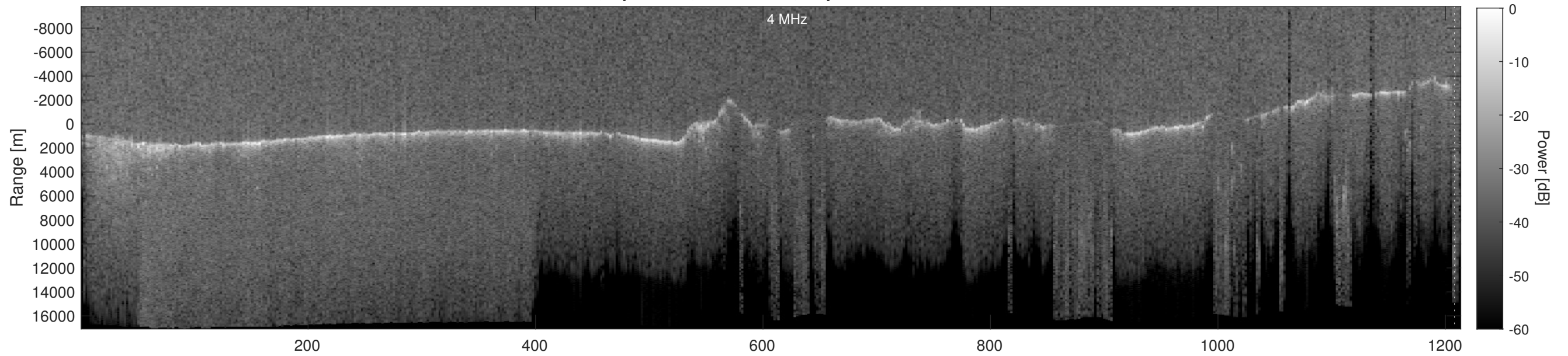
Orbit 15736, Depth-Corrected Cluttergram
