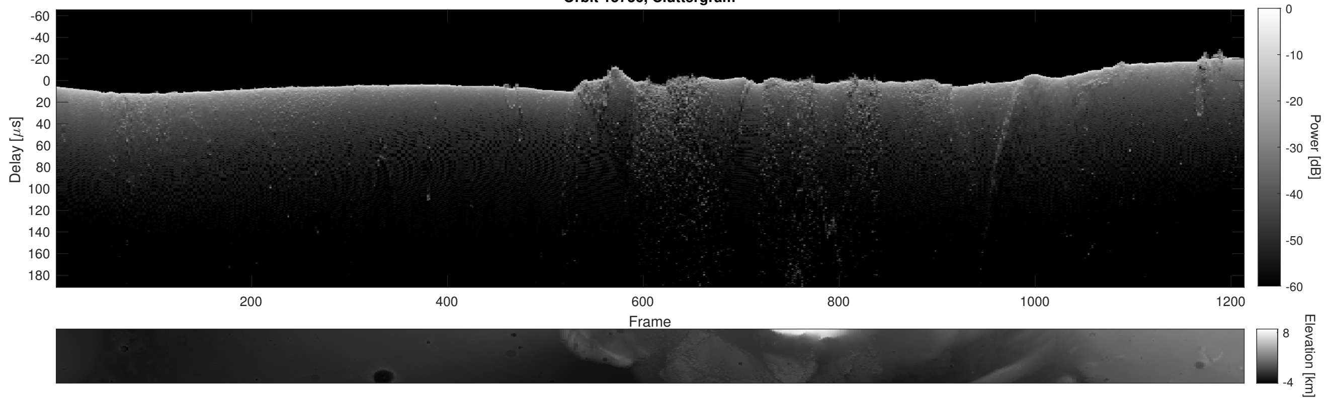
Orbit 15736, Cluttergram
