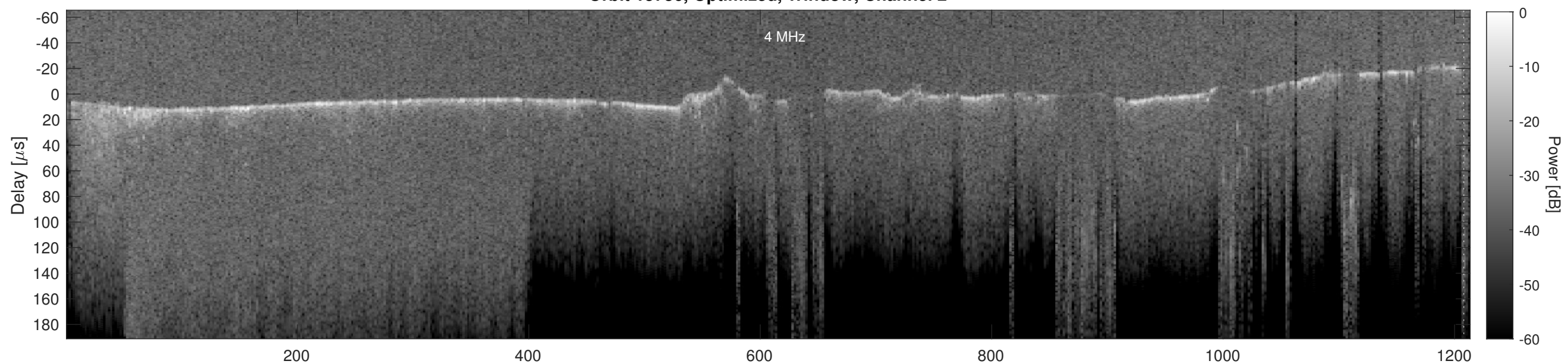
Orbit 15736, Cluttergram
