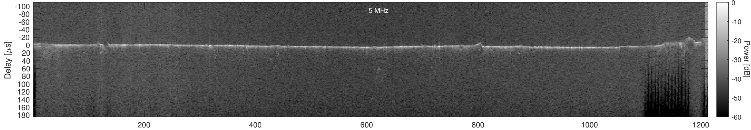
Orbit 15740, Cluttergram
