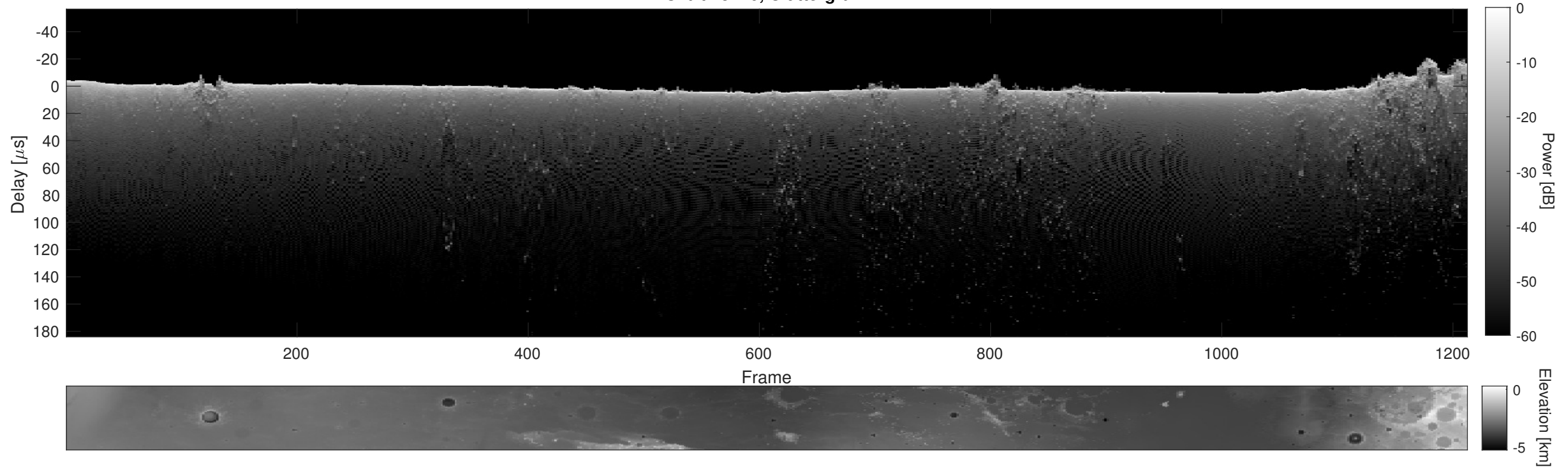
Orbit 15740, Cluttergram
