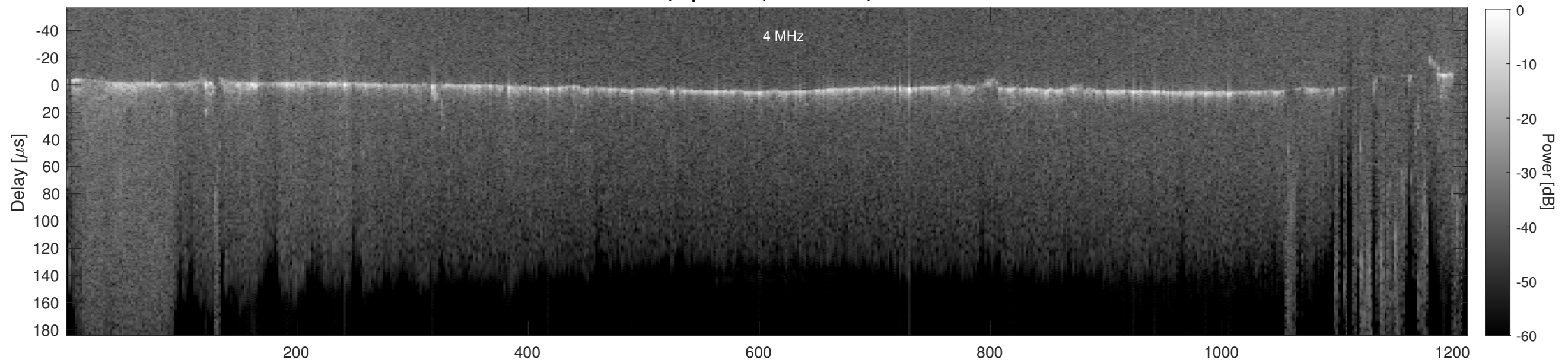
Orbit 15740, Cluttergram
