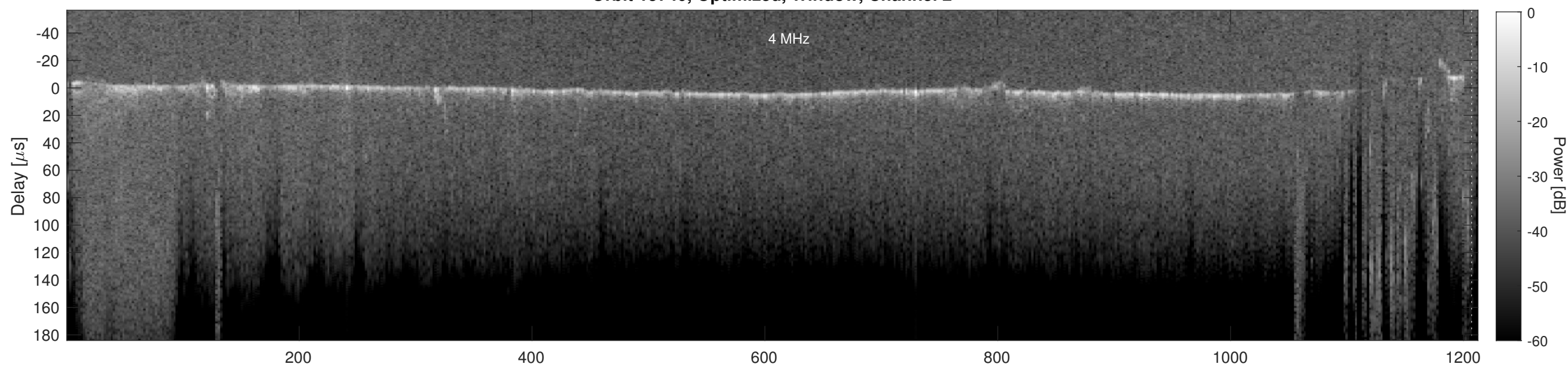
Orbit 15740, Cluttergram
