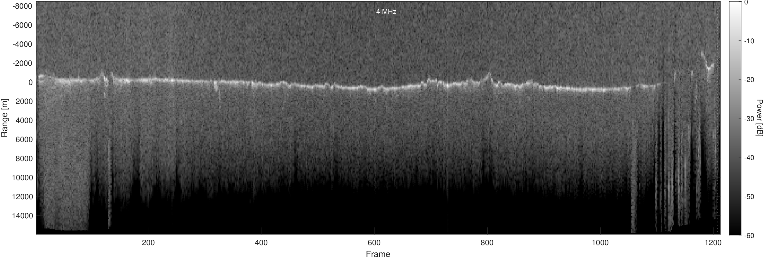
Orbit 15740, Optimized, Window, Depth-Corrected, Channel 2
