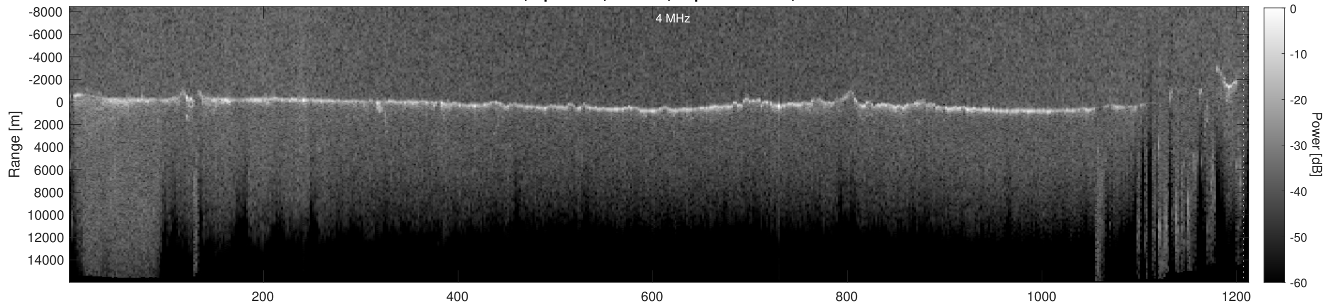
Orbit 15740, Depth-Corrected Cluttergram
