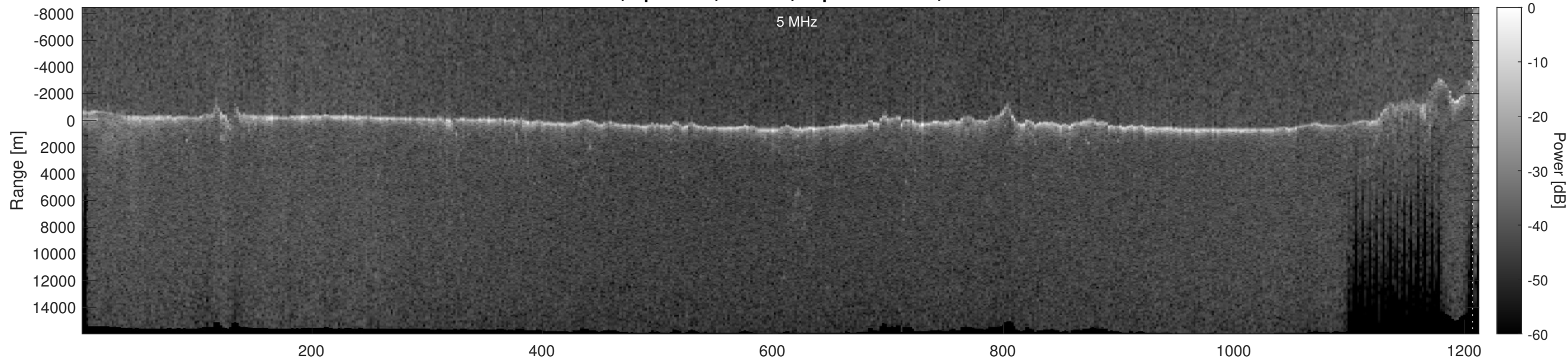
Orbit 15740, Optimized, Window, Depth-Corrected, Channel 2
