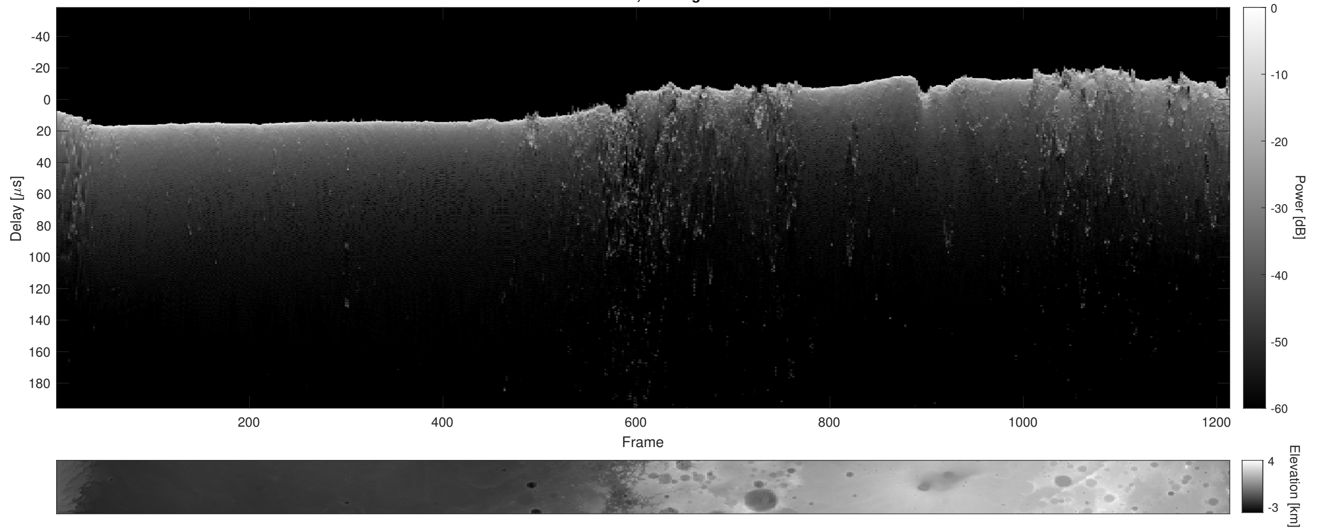
Orbit 15741, Cluttergram
