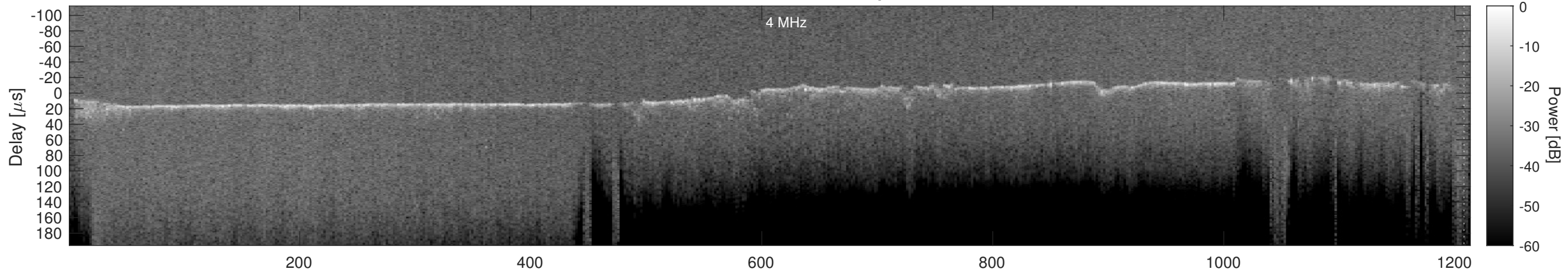
Orbit 15741, Cluttergram
