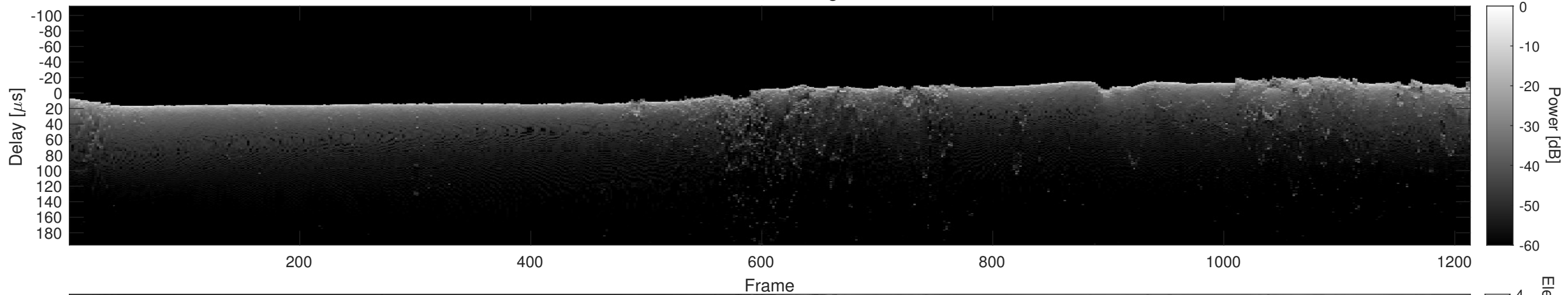
Orbit 15741, Cluttergram
