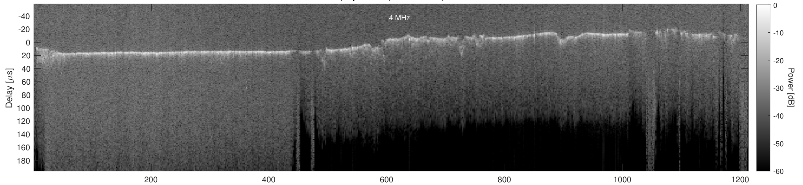
Orbit 15741, Cluttergram
