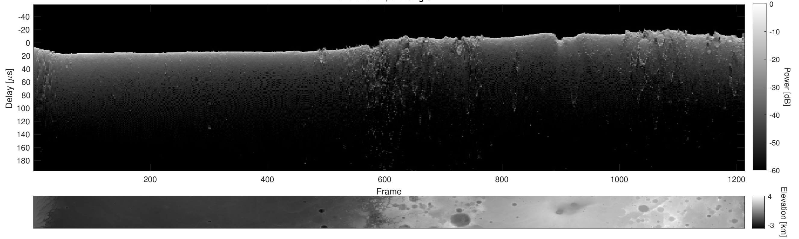
Orbit 15741, Cluttergram
