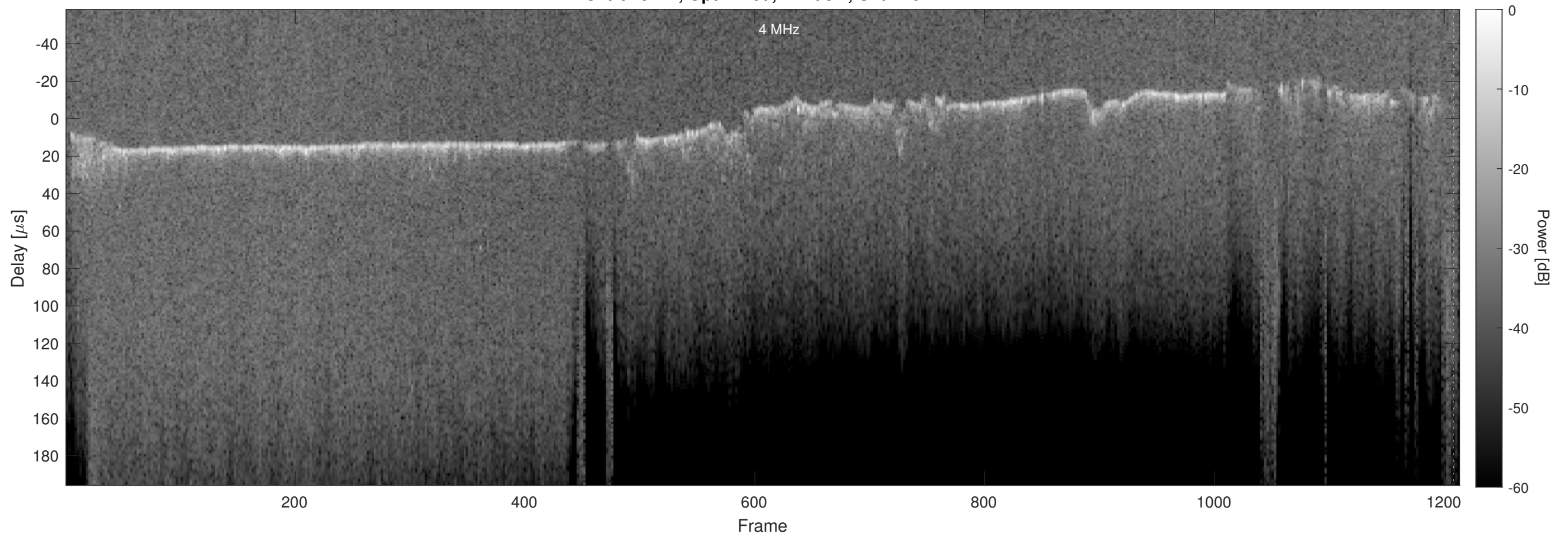
Orbit 15741, Optimized, Window, Channel 2
