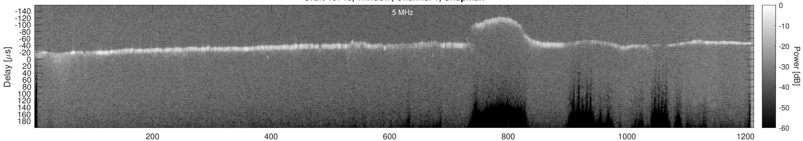
Orbit 15743, Window, Channel 1, Optimized
