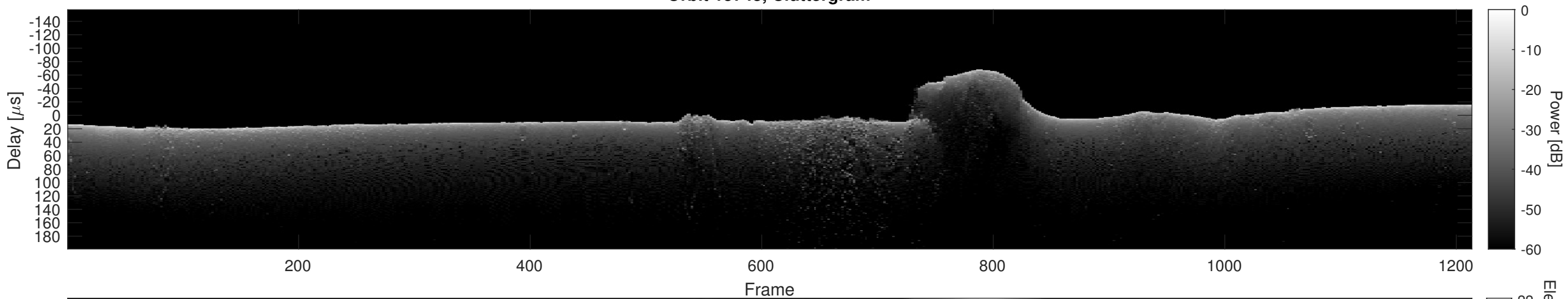
Orbit 15743, Cluttergram
