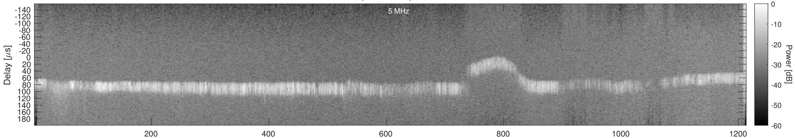
Orbit 15743, Window, Channel 1, Chapman
