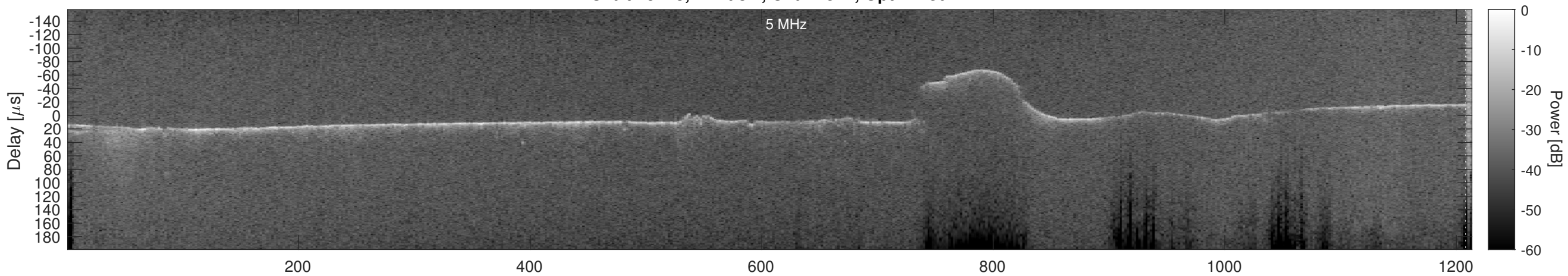
Orbit 15743, Cluttergram
