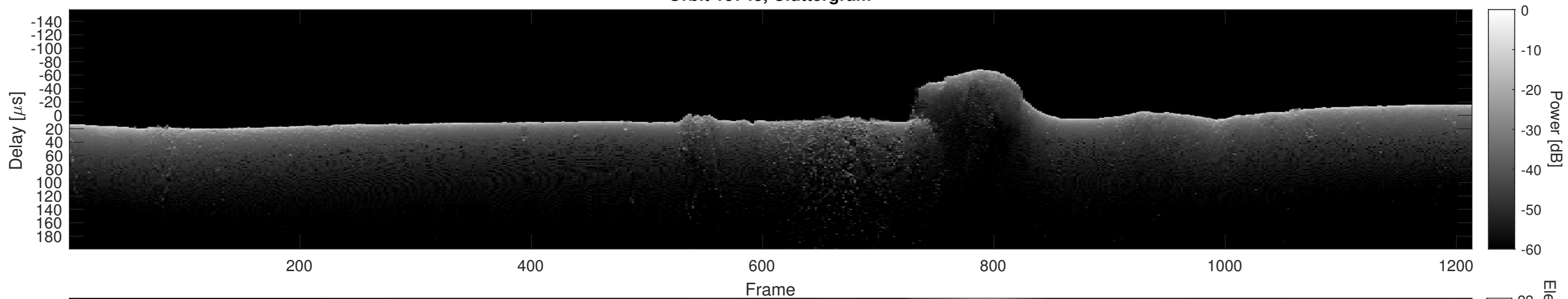
Orbit 15743, Cluttergram
