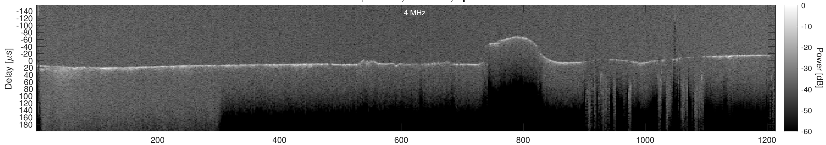
Orbit 15743, Cluttergram
