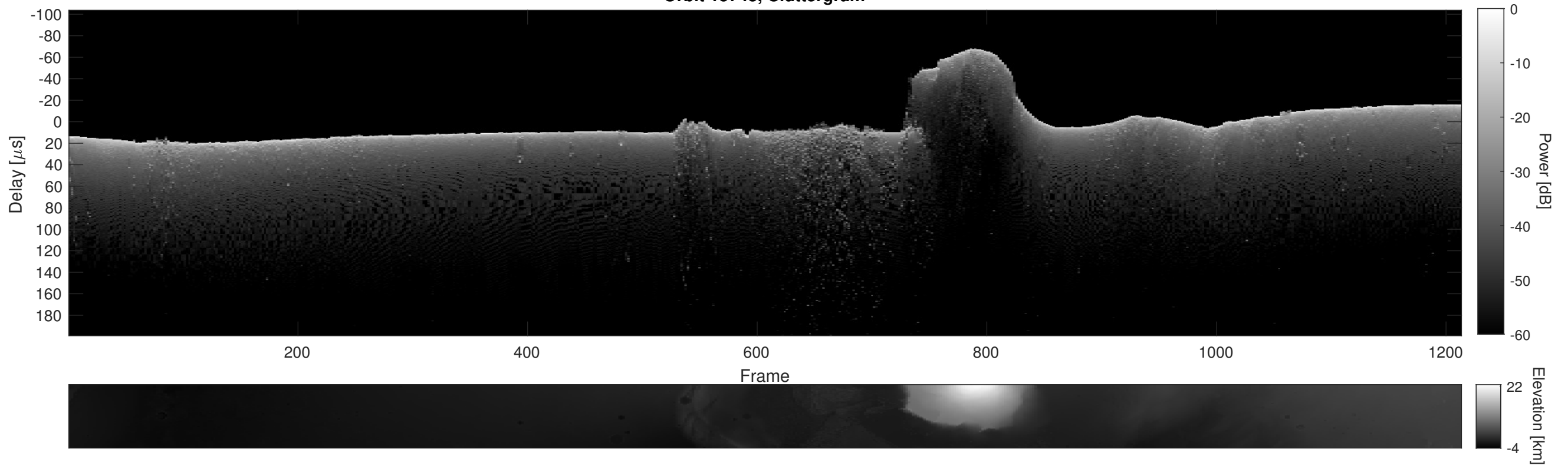
Orbit 15743, Cluttergram
