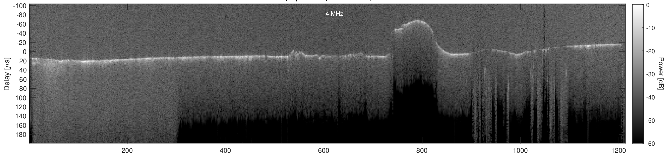
Orbit 15743, Cluttergram
