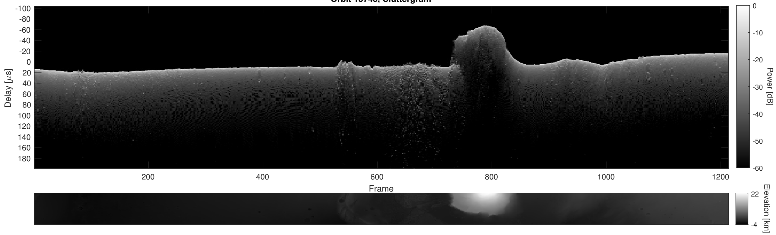
Orbit 15743, Cluttergram
