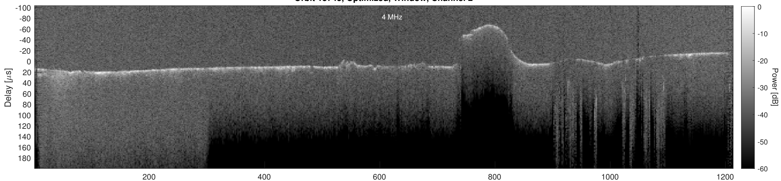
Orbit 15743, Cluttergram
