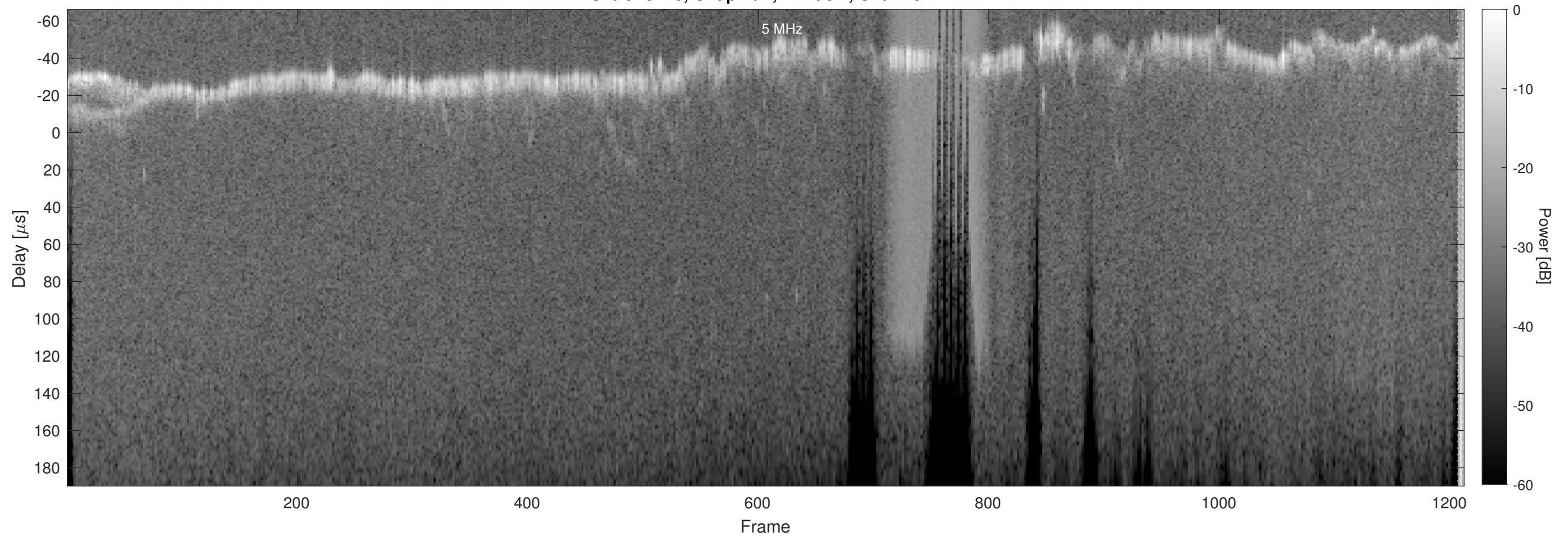
Orbit 15745, Chapman, Window, Channel 2
