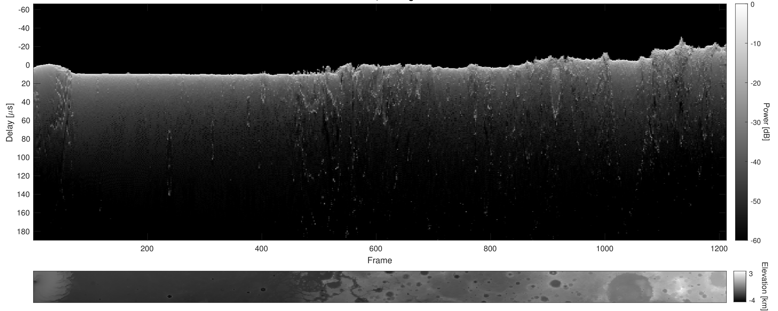
Orbit 15745, Cluttergram
