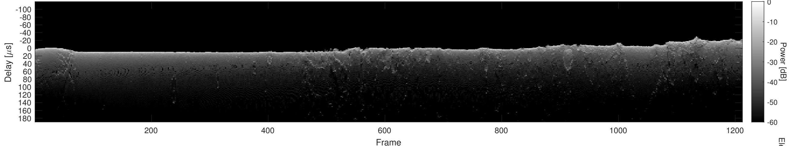
Orbit 15745, Cluttergram
