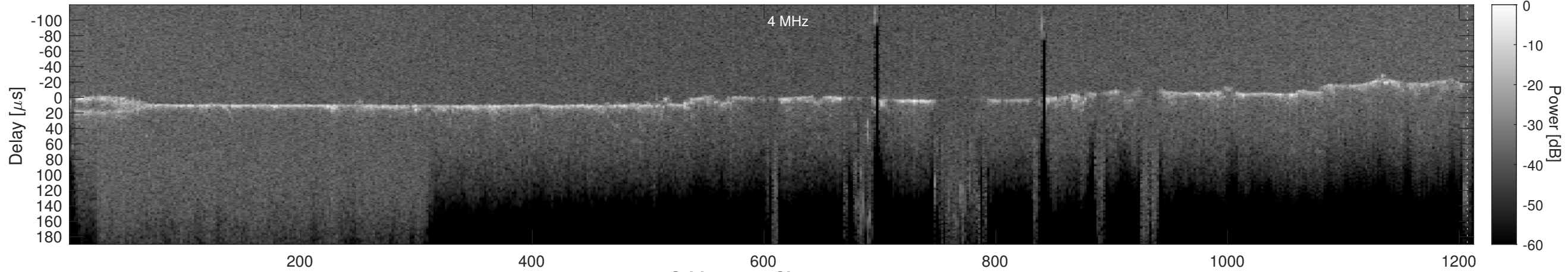
Orbit 15745, Cluttergram
