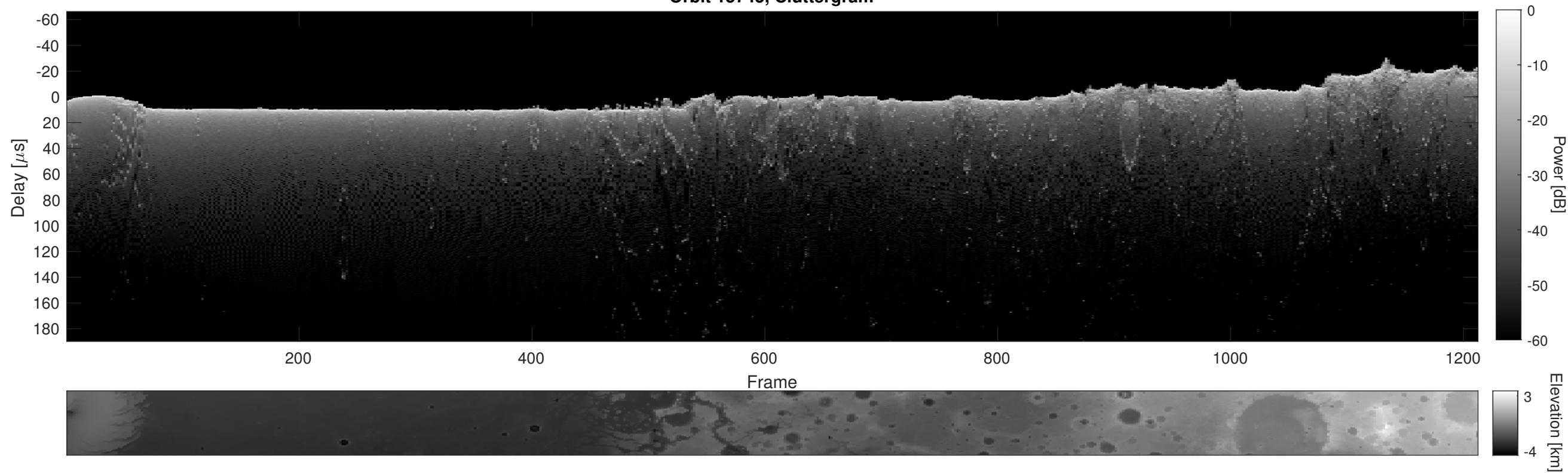
Orbit 15745, Cluttergram
