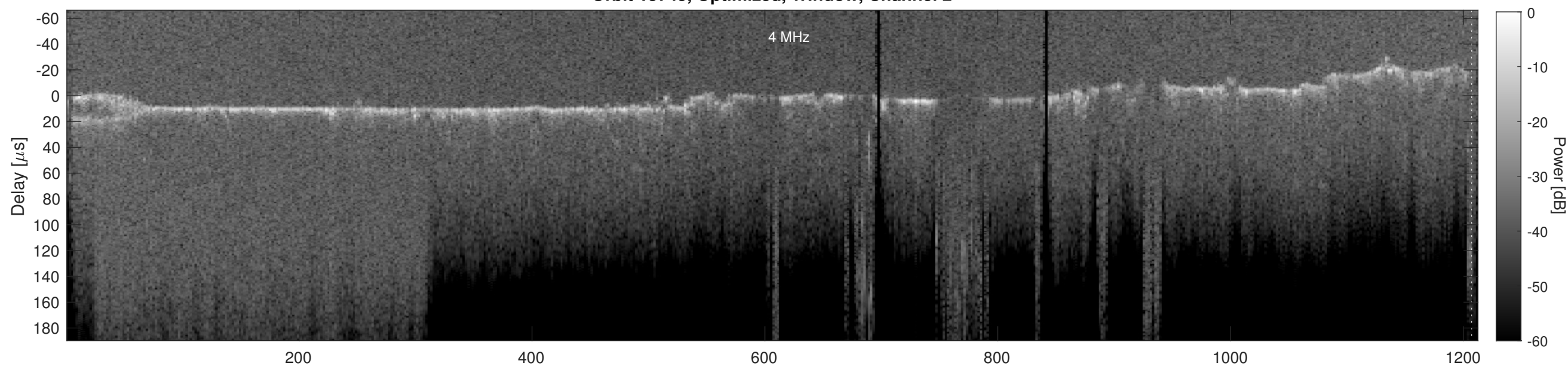
Orbit 15745, Cluttergram
