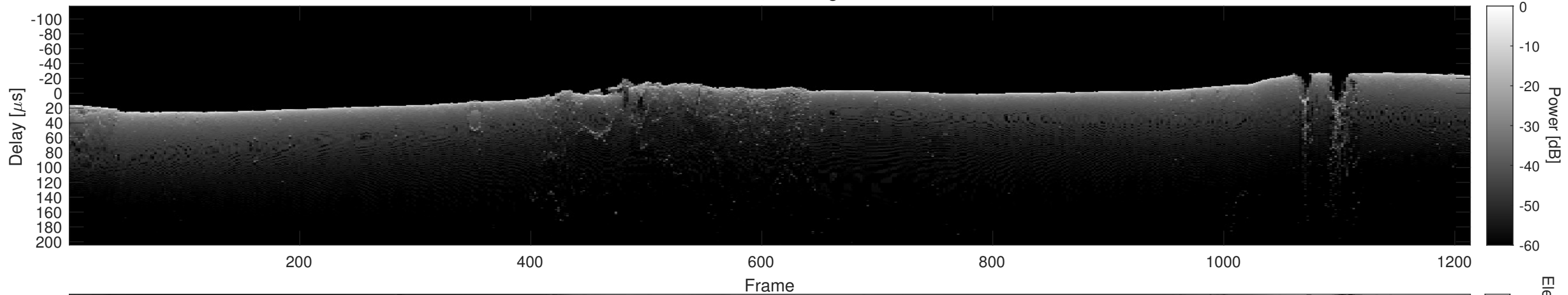
Orbit 15746, Cluttergram
