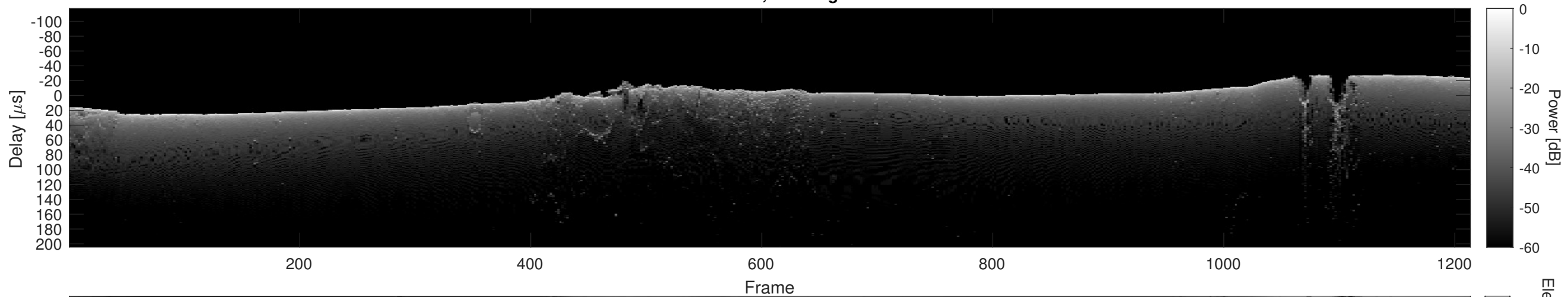
Orbit 15746, Cluttergram
