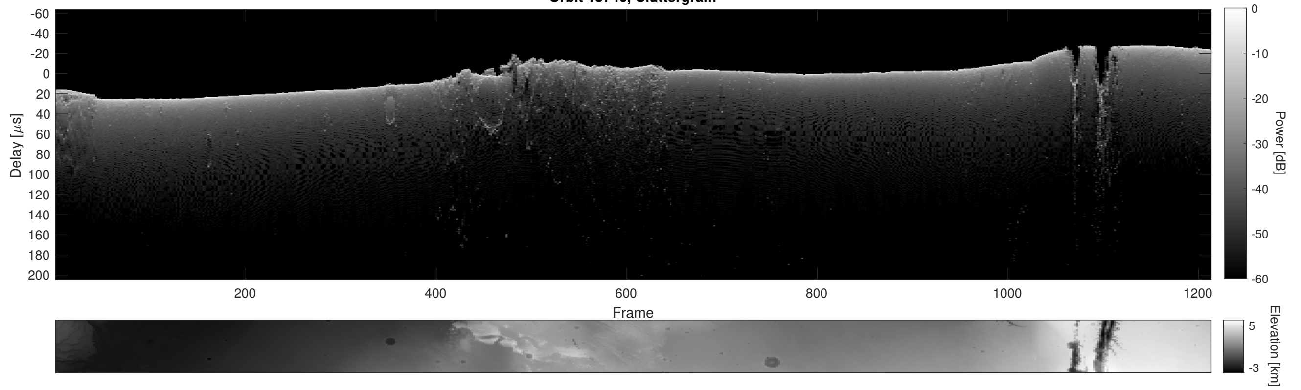
Orbit 15746, Cluttergram
