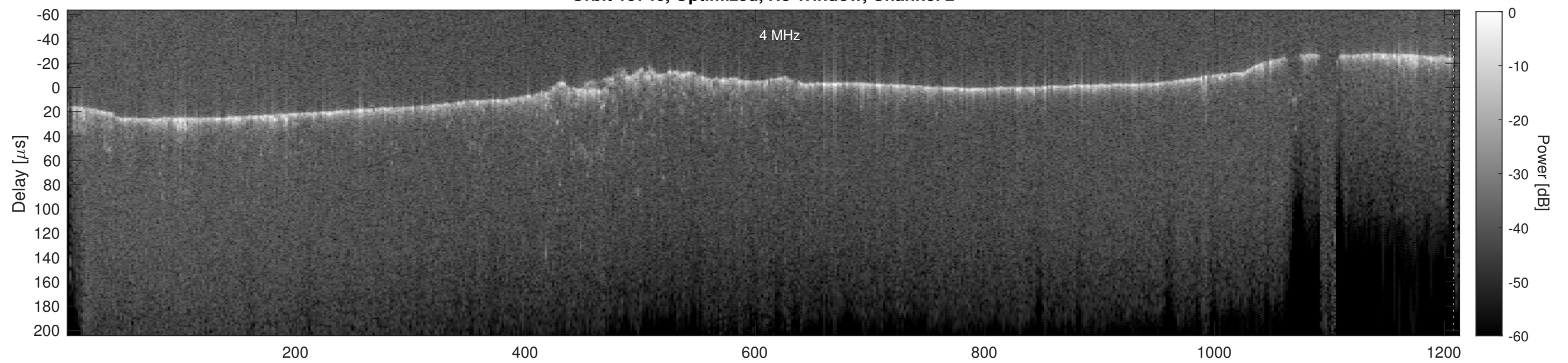
Orbit 15746, Cluttergram
