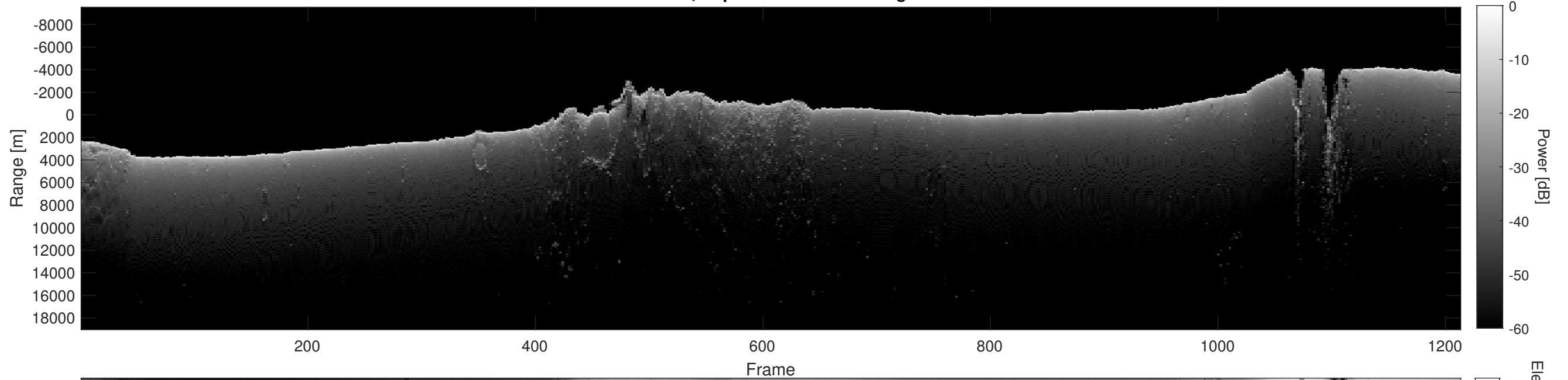
Orbit 15746, Depth-Corrected Cluttergram
