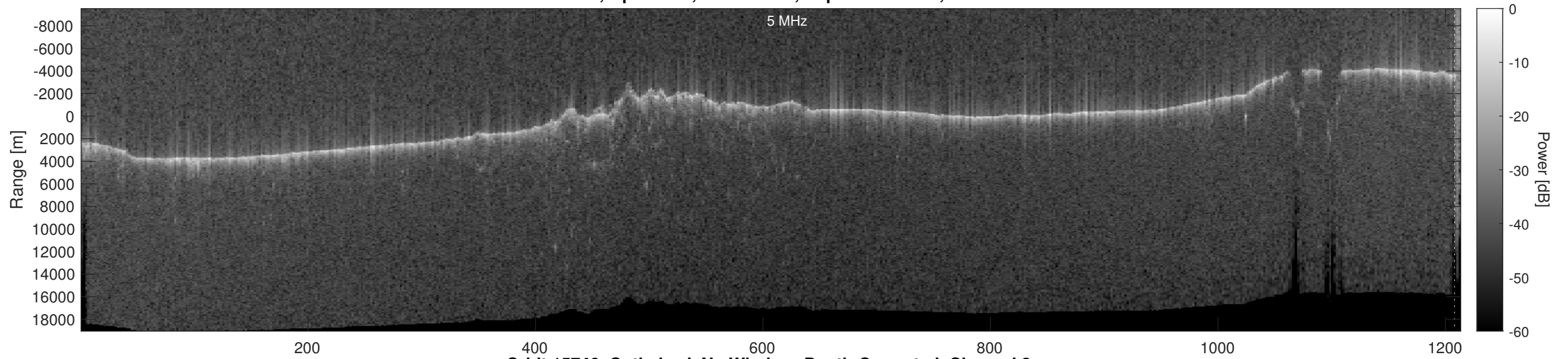
Orbit 15746, Optimized, No Window, Depth-Corrected, Channel 2
