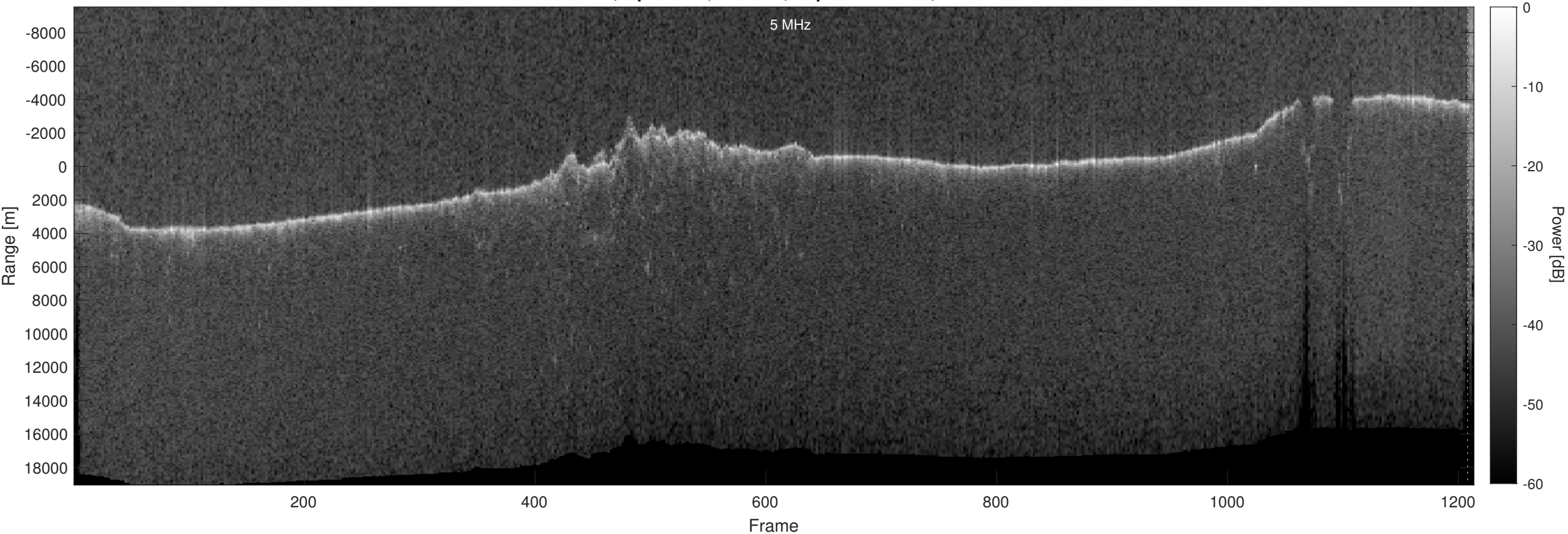
Orbit 15746, Optimized, Window, Depth-Corrected, Channel 2
