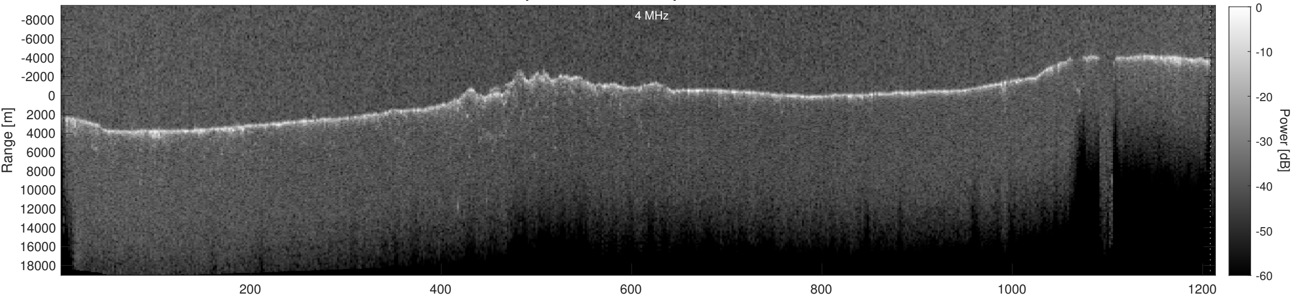
Orbit 15746, Depth-Corrected Cluttergram
