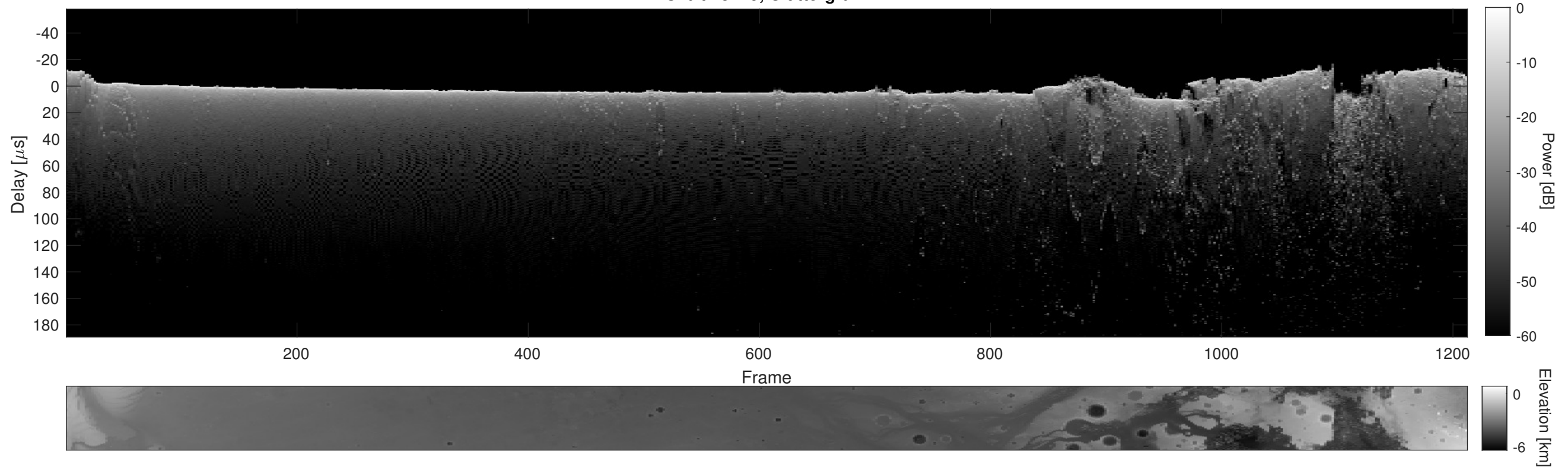
Orbit 15749, Cluttergram
