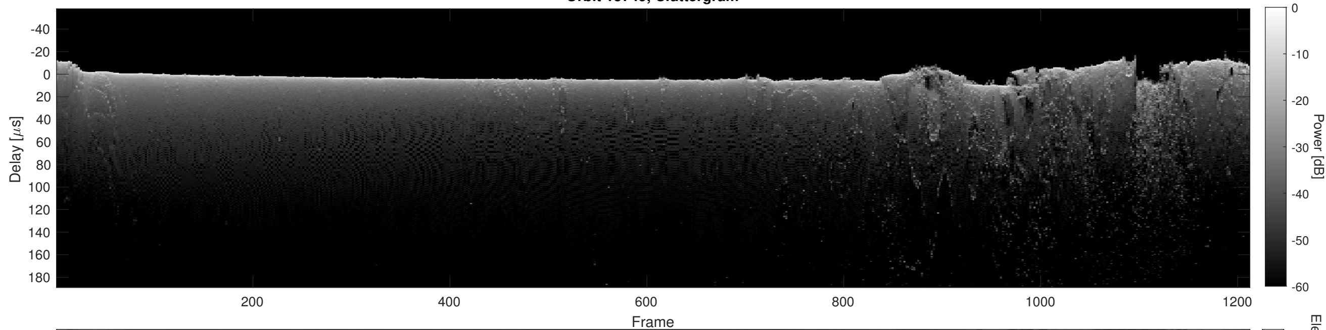
Orbit 15749, Cluttergram
