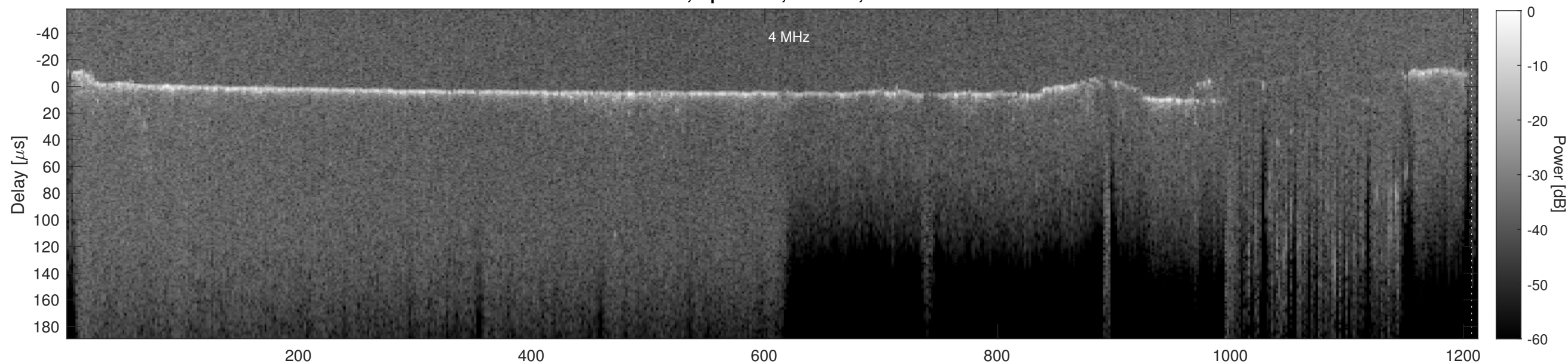
Orbit 15749, Cluttergram
