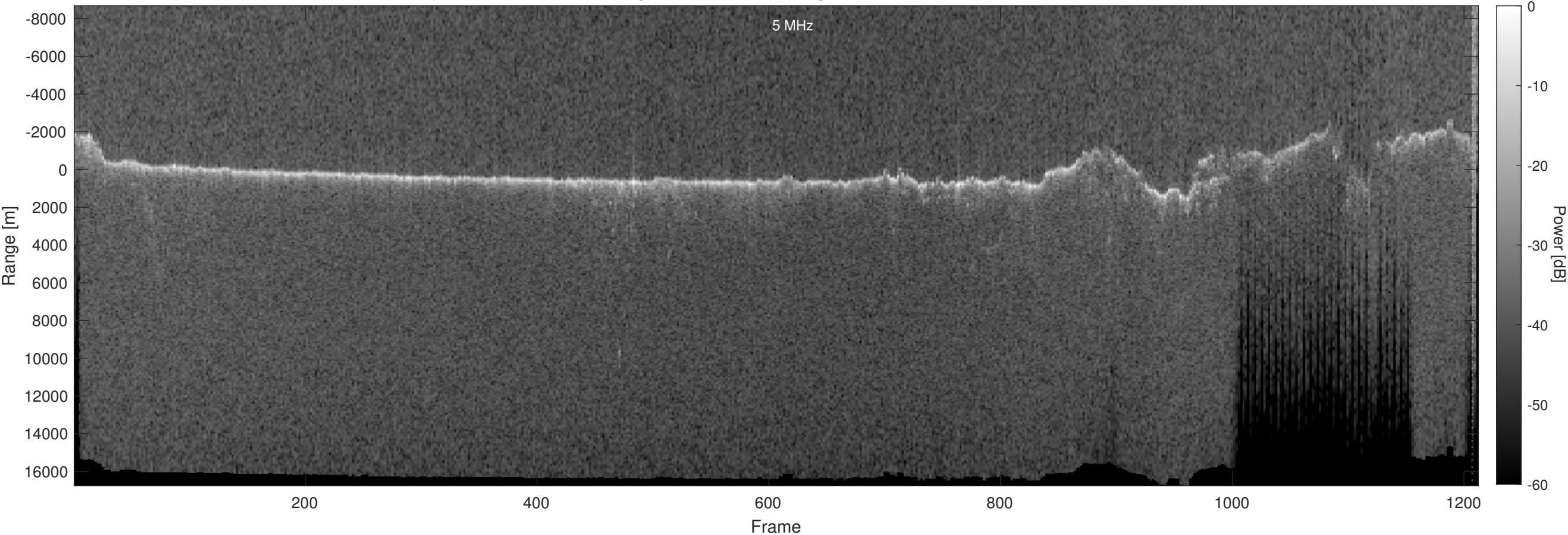
Orbit 15749, Optimized, Window, Depth-Corrected, Channel 2
