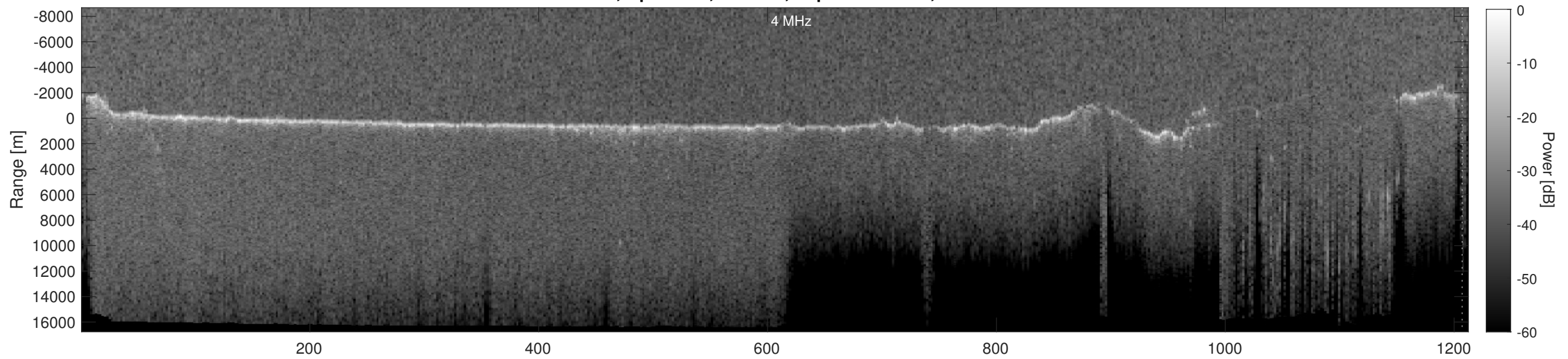
Orbit 15749, Depth-Corrected Cluttergram
