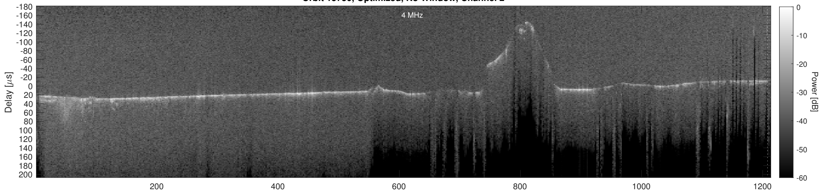
Orbit 15750, Cluttergram
