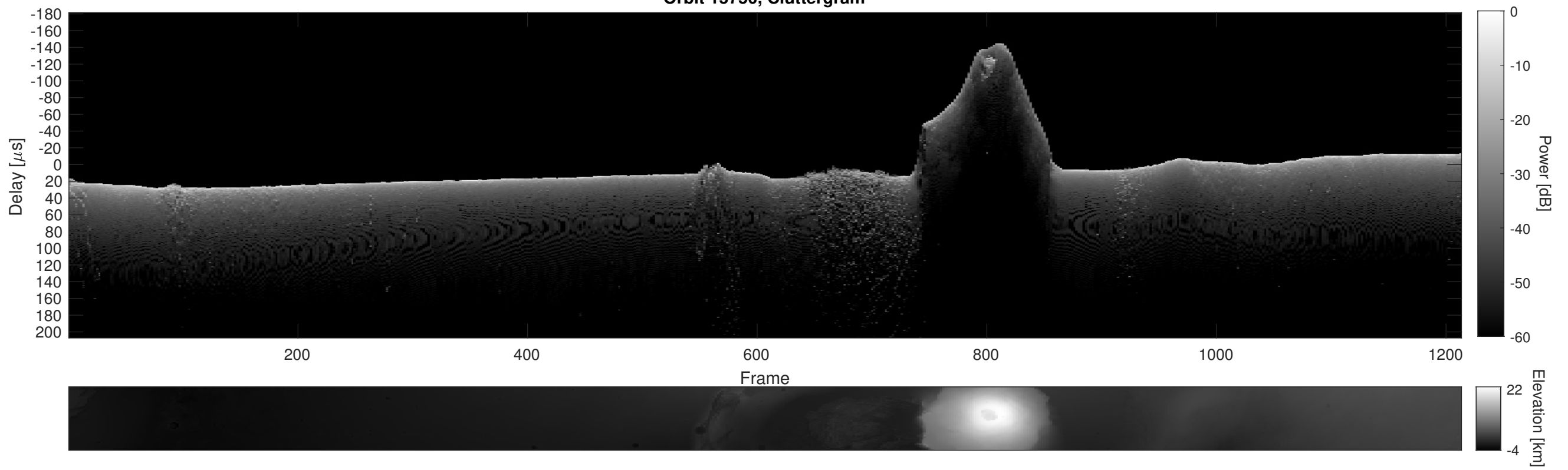
Orbit 15750, Cluttergram
