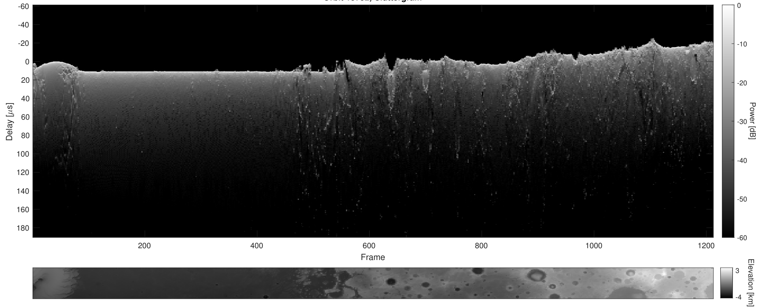
Orbit 15752, Cluttergram
