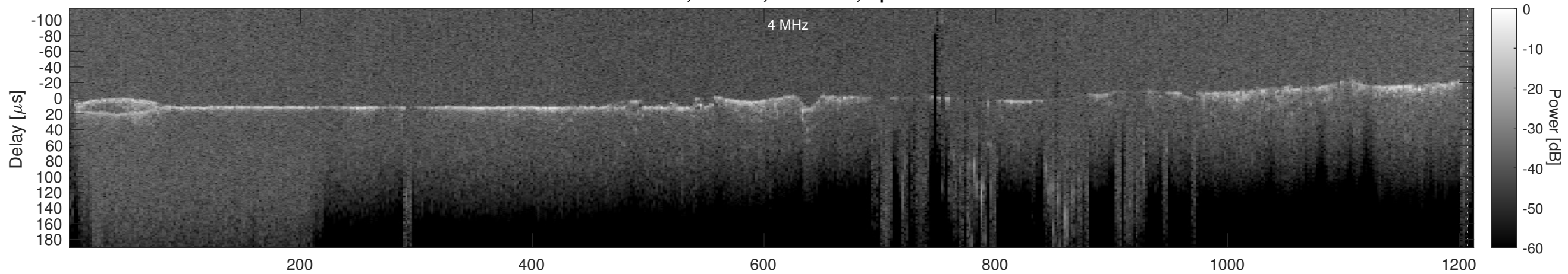
Orbit 15752, Cluttergram
