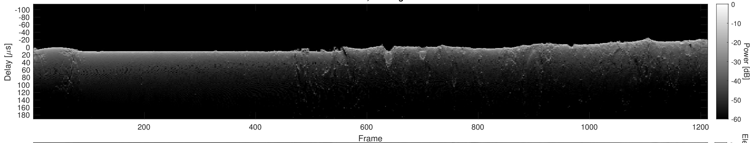
Orbit 15752, Cluttergram
