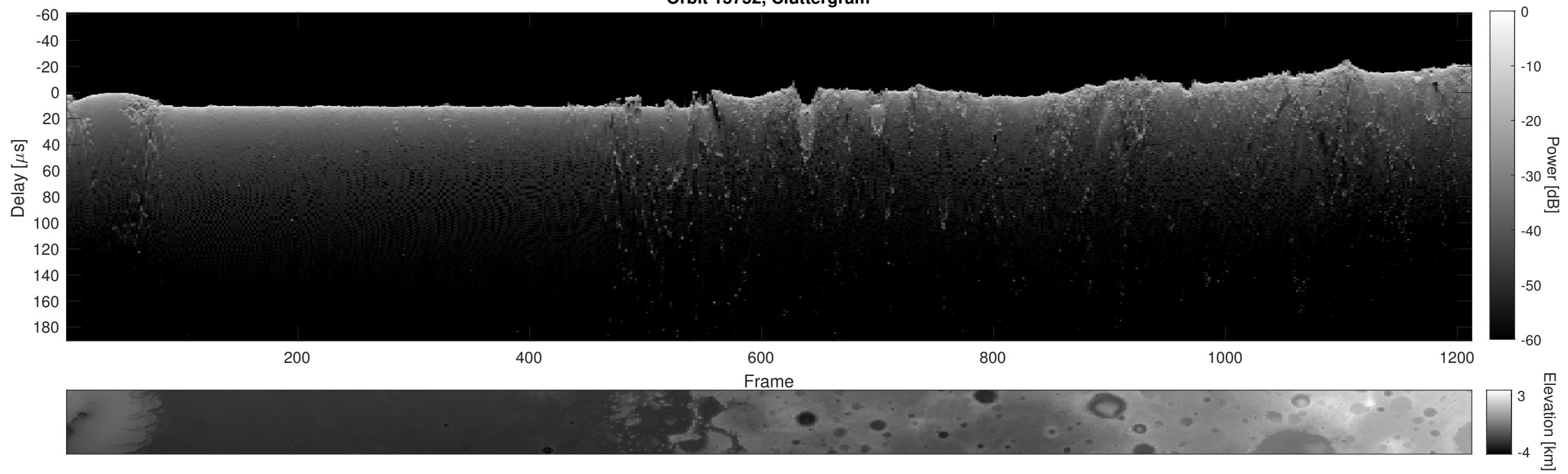
Orbit 15752, Cluttergram
