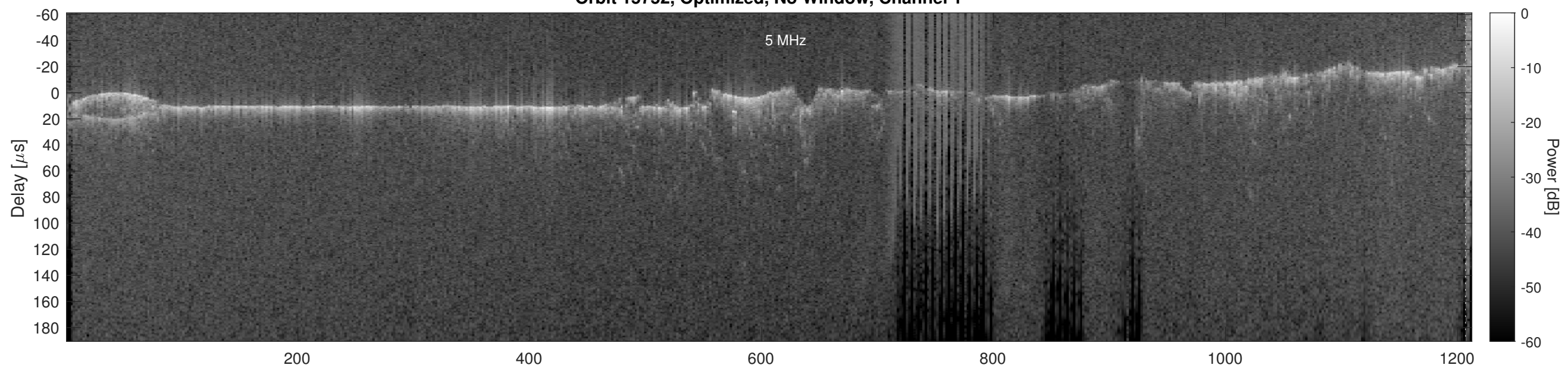
Orbit 15752, Optimized, No Window, Channel 2
