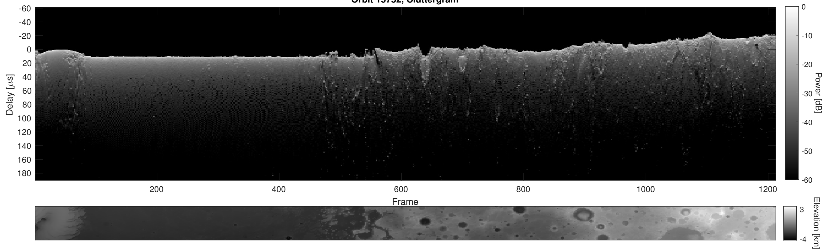
Orbit 15752, Cluttergram
