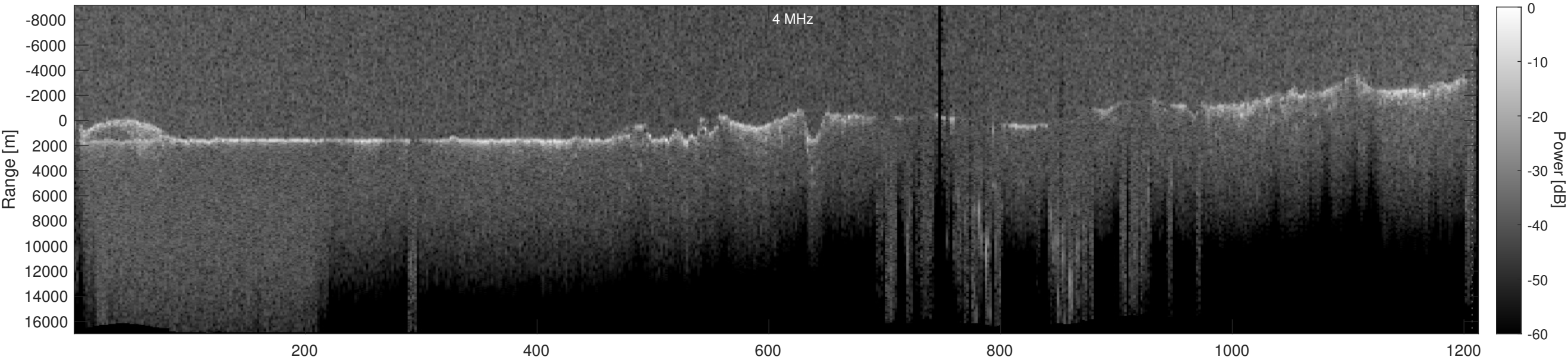
Orbit 15752, Depth-Corrected Cluttergram
