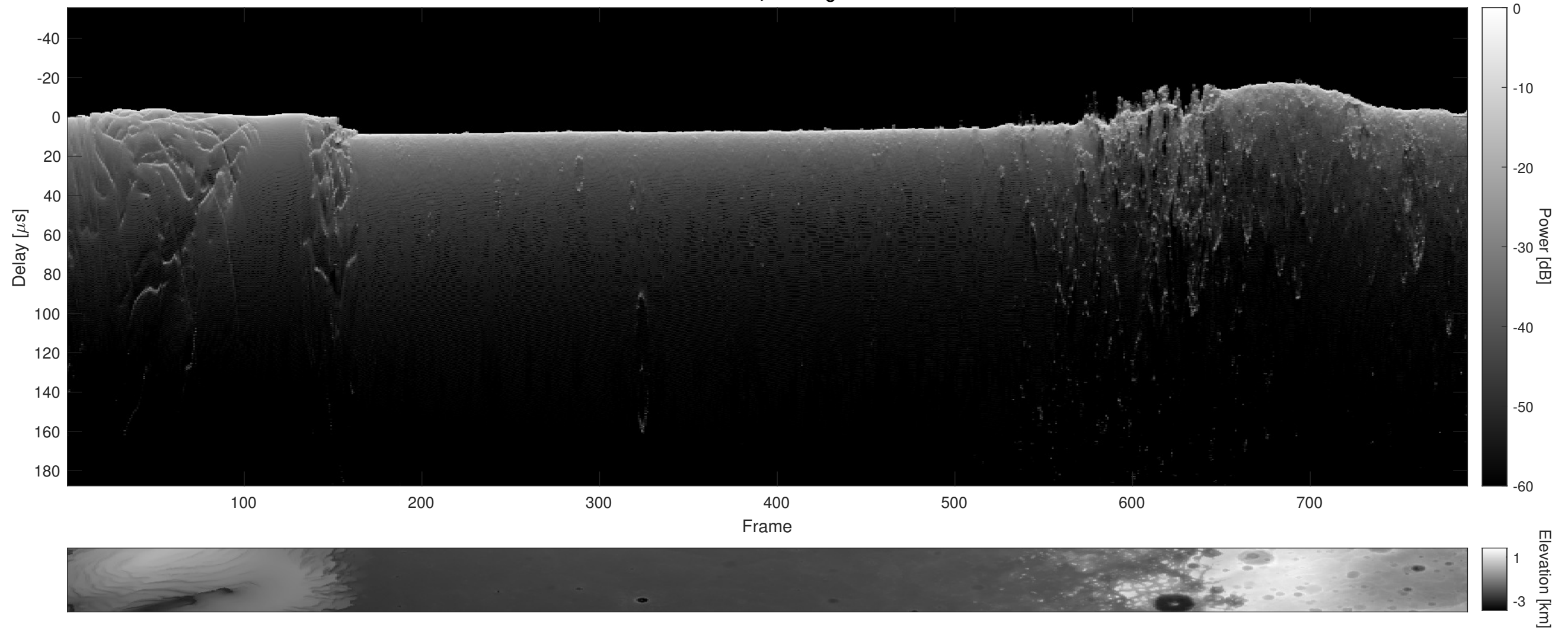
Orbit 15801, Cluttergram
