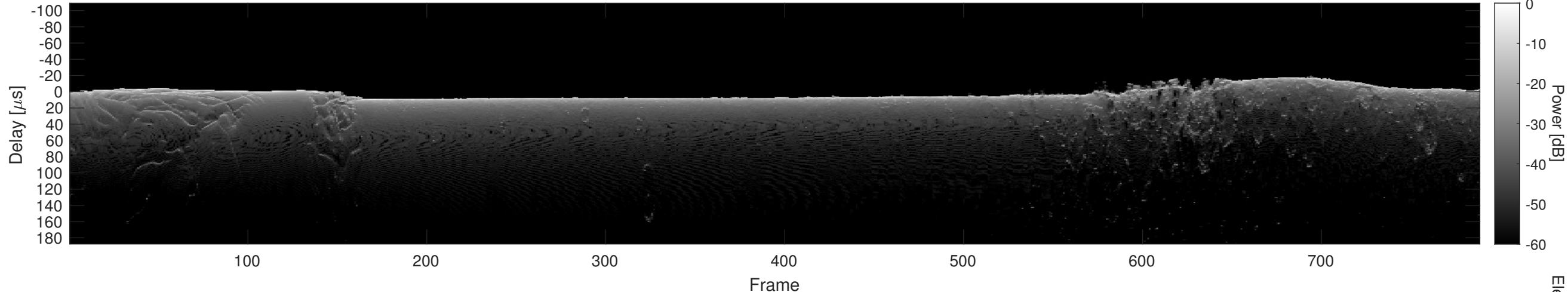
Orbit 15801, Cluttergram
