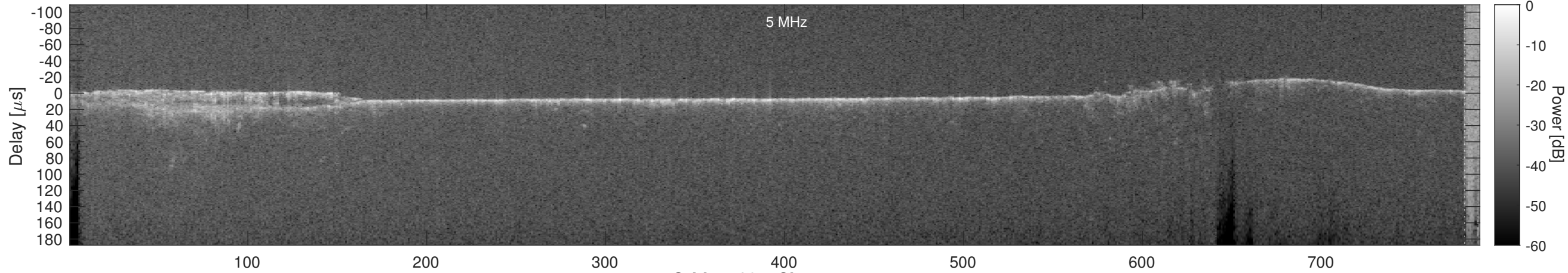
Orbit 15801, Cluttergram
