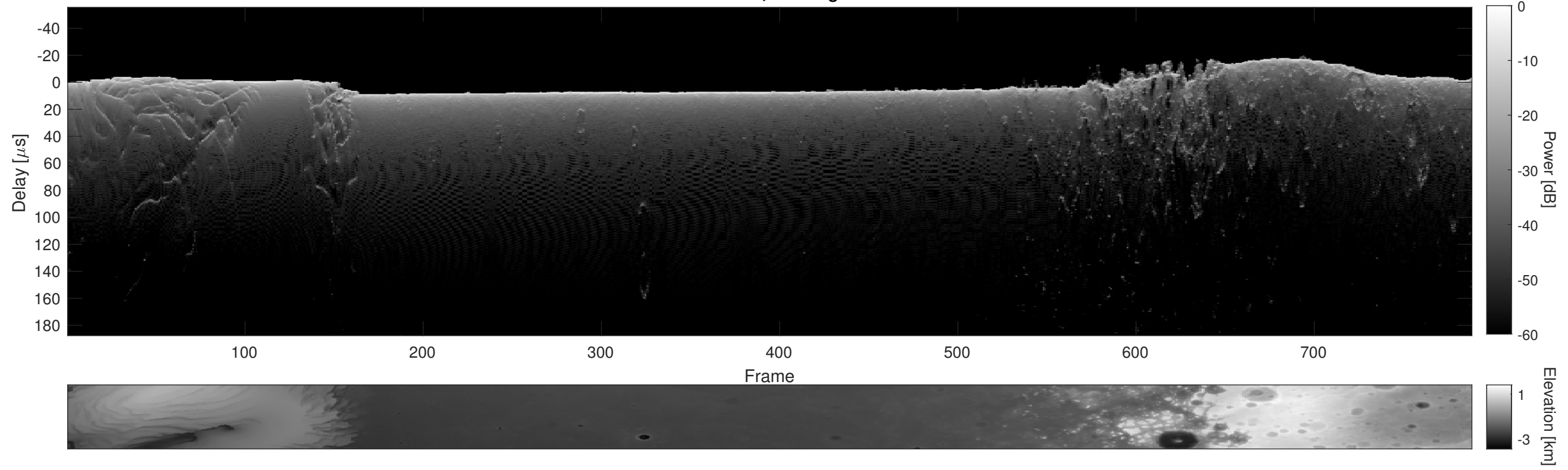
Orbit 15801, Cluttergram
