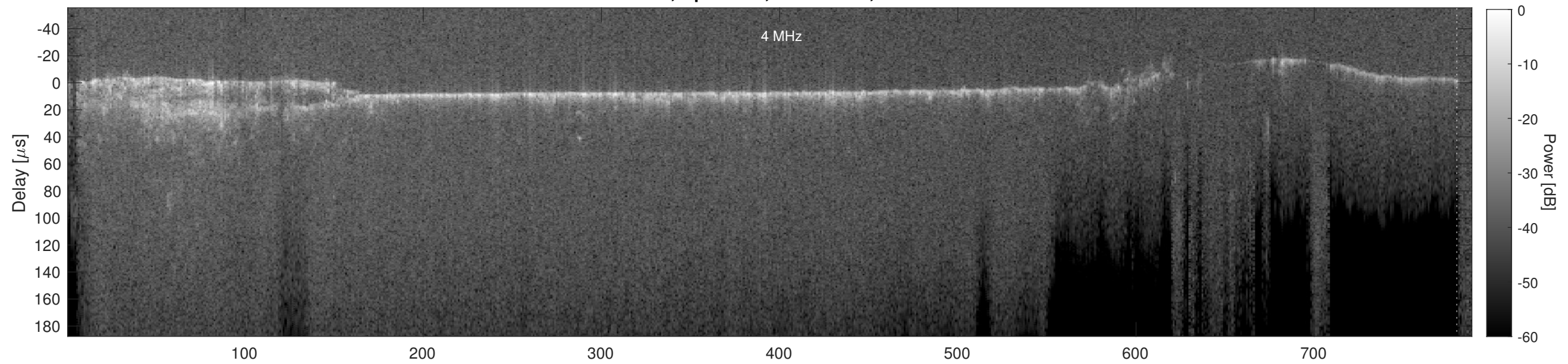
Orbit 15801, Cluttergram
