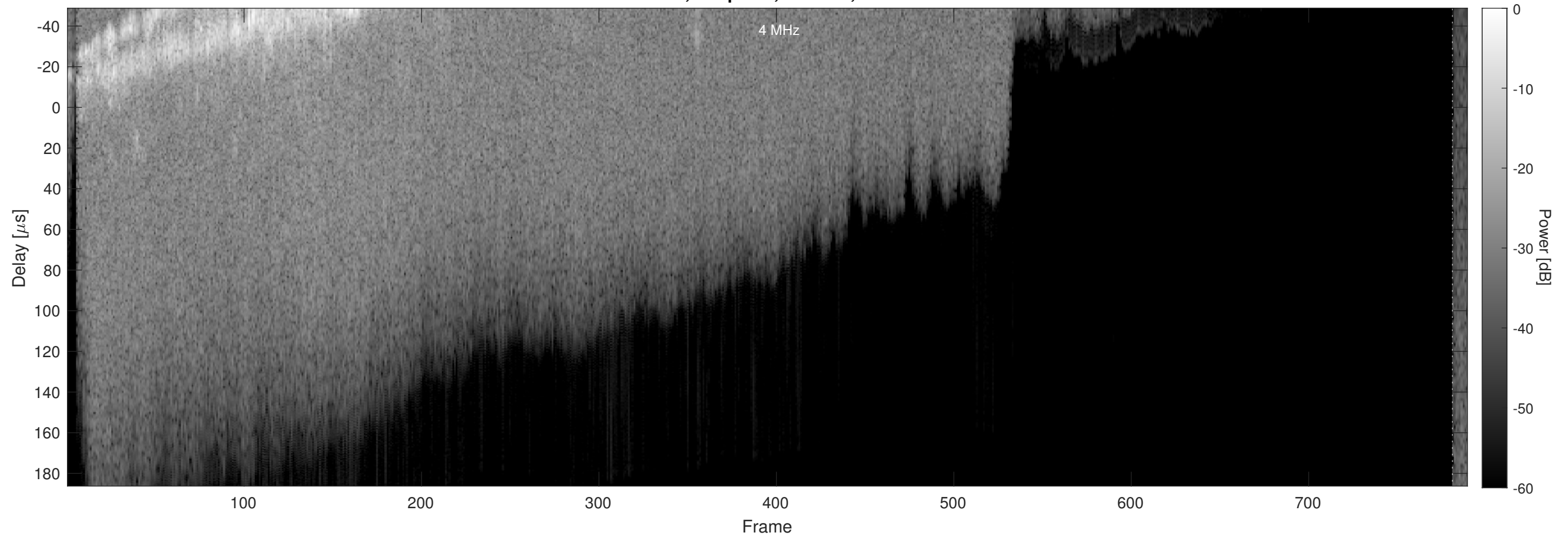
Orbit 15804, Chapman, Window, Channel 2
