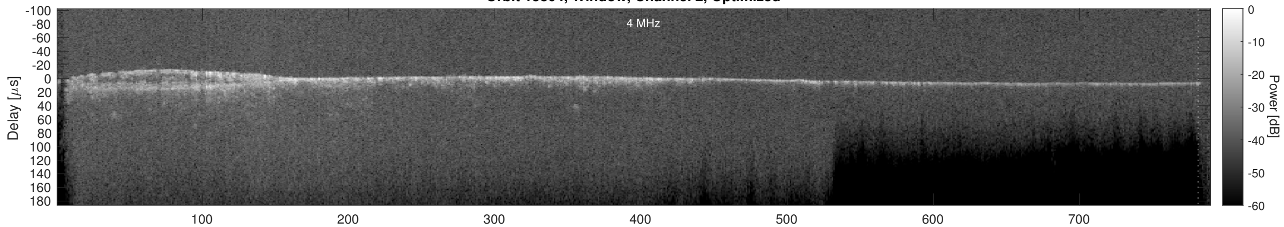
Orbit 15804, Cluttergram
