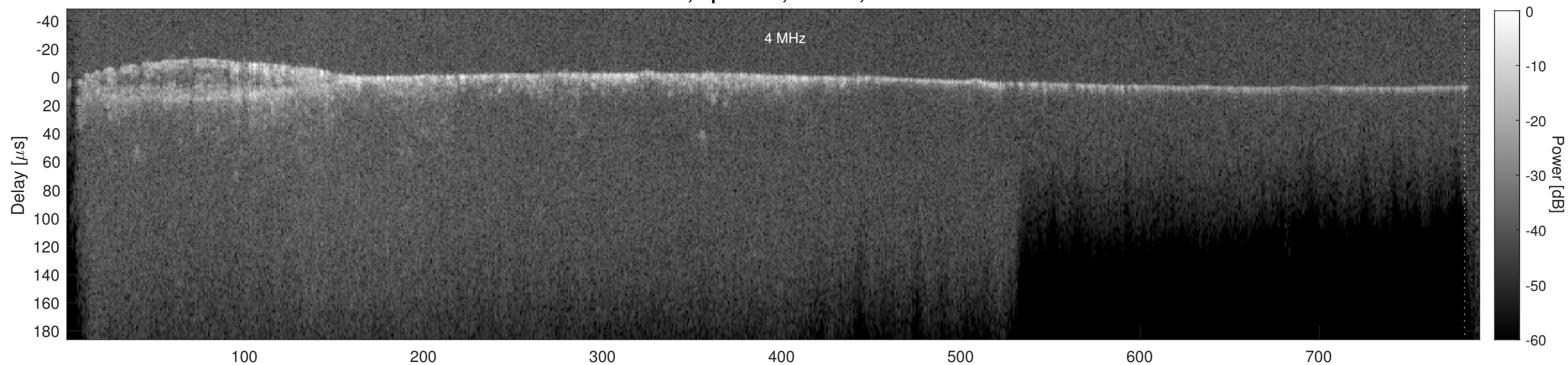
Orbit 15804, Cluttergram
