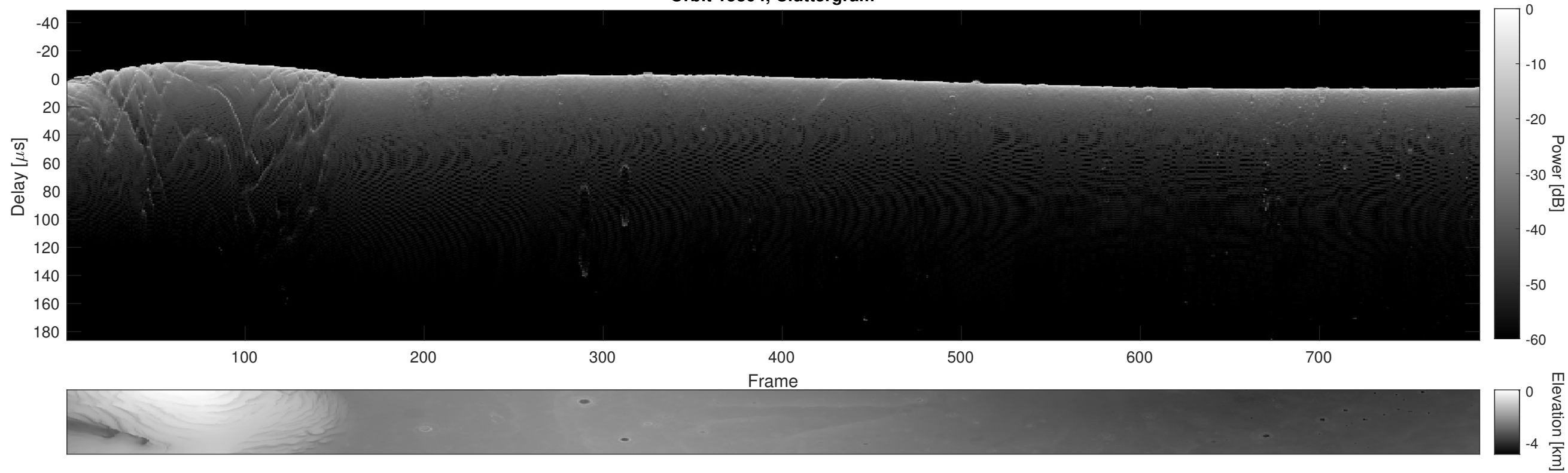
Orbit 15804, Cluttergram
